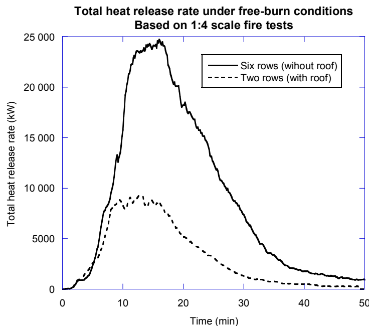
Figure 7 The potential severity of the test set-up based on down-scaled fire tests.
