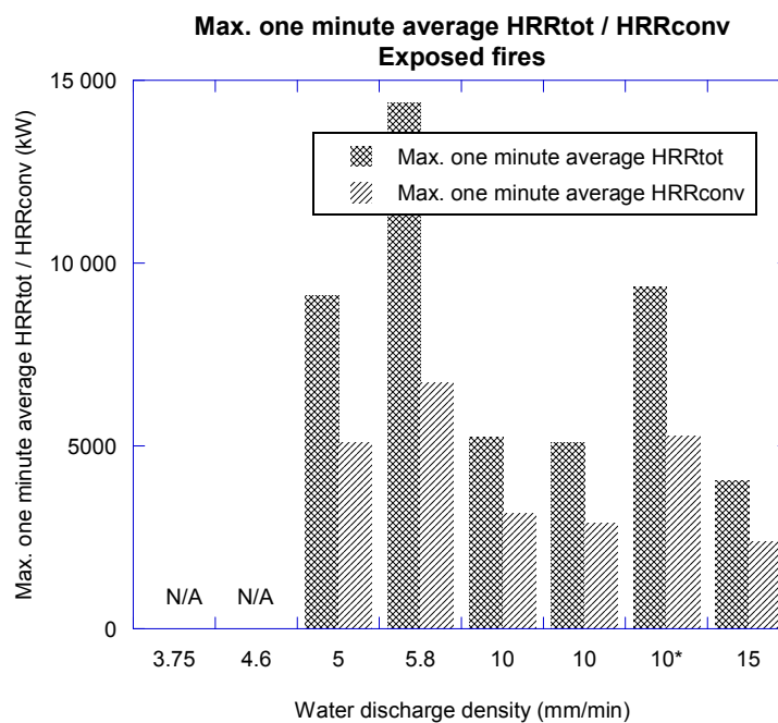
Figure 26 The maximum one minute average total and convective heat release rate for the fire tests without the roof of the trailer mock-up. The (*) indicates the test with delayed activation of the system.
