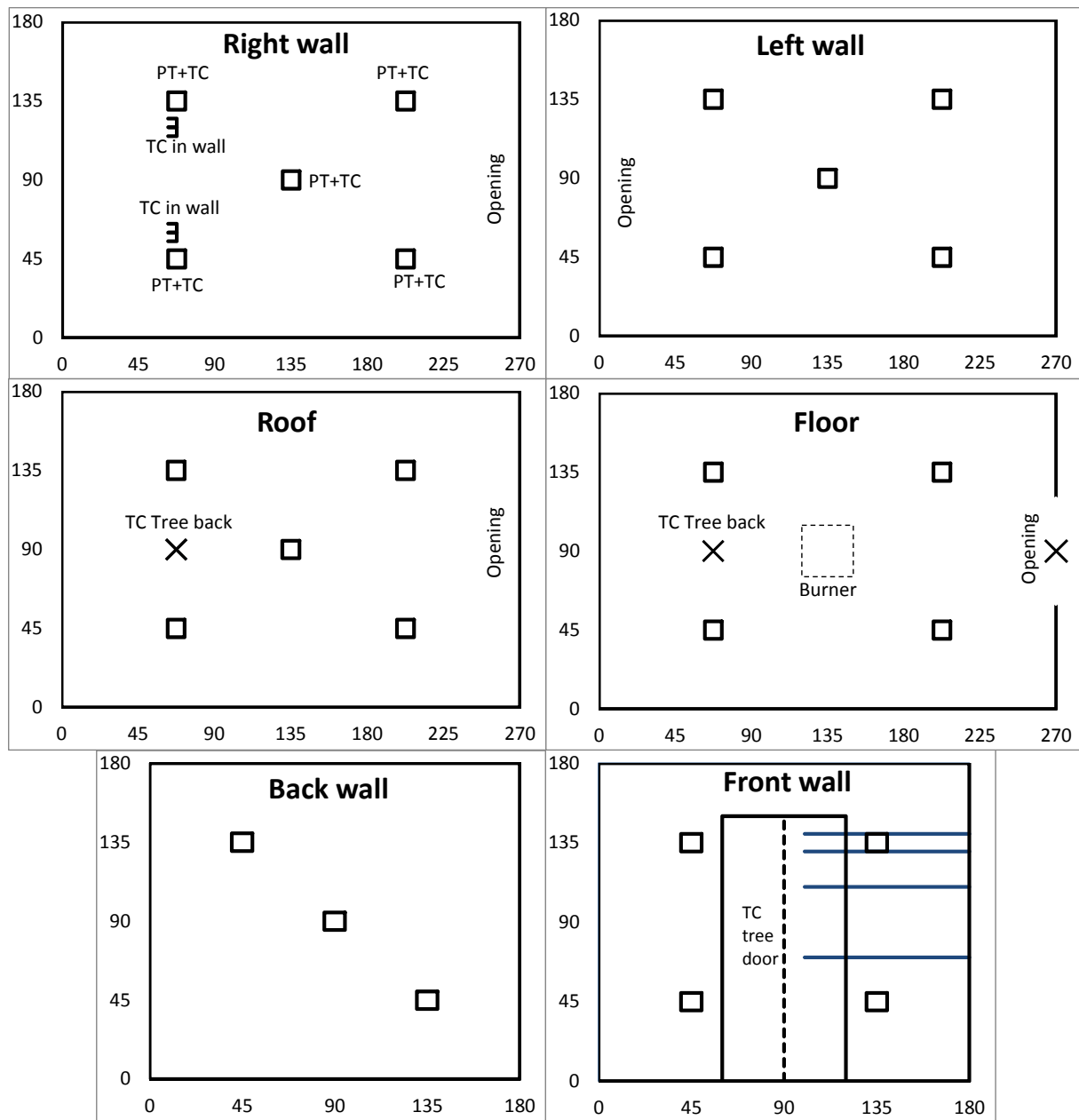
Figure 8 The instrumentation at the inside of the enclosure for test series A. The distances are in cm. All squares are PT only unless stated otherwise. The back TC tree spans from roof to floor and the door TC tree from top to bottom of the opening. O 2 gas measurements are measured in the opening a distance 100, 200, 400 and 800 mm from the top of the opening.
