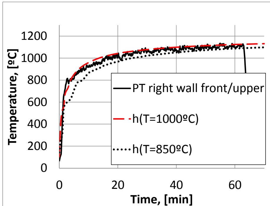
Figure 25. Comparison of calculated temperatures with measured higher temperature during experiments – Case A1.
