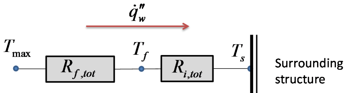
Figure 5 Electric circuit analogy model of a fire compartment with infinitely thick walls.
