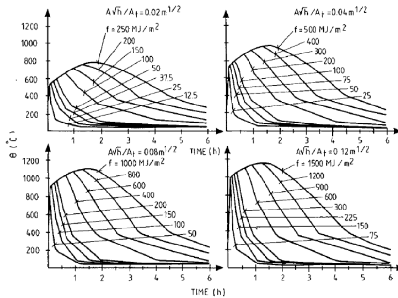
Figure 1. Temperature –time dependence of a fully developed fire for various fire load densities and opening factors (adapted from (Pettersson, et al., 1976))
