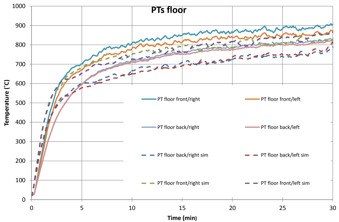
Figure 17 Plate thermometers on the floor.
