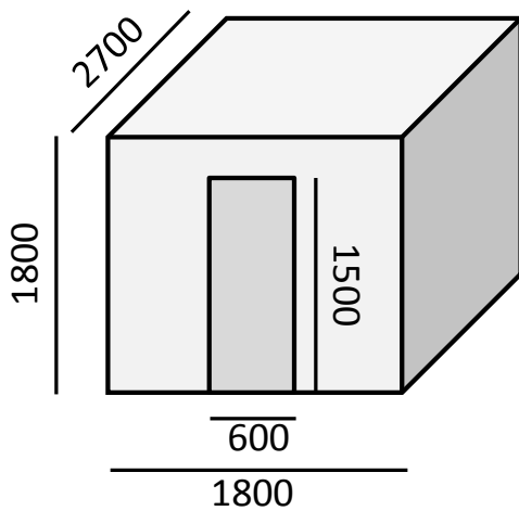
Figure 7 Left: inner dimensions of the enclosure. Right: test object of 100 mm lightweight concrete.
