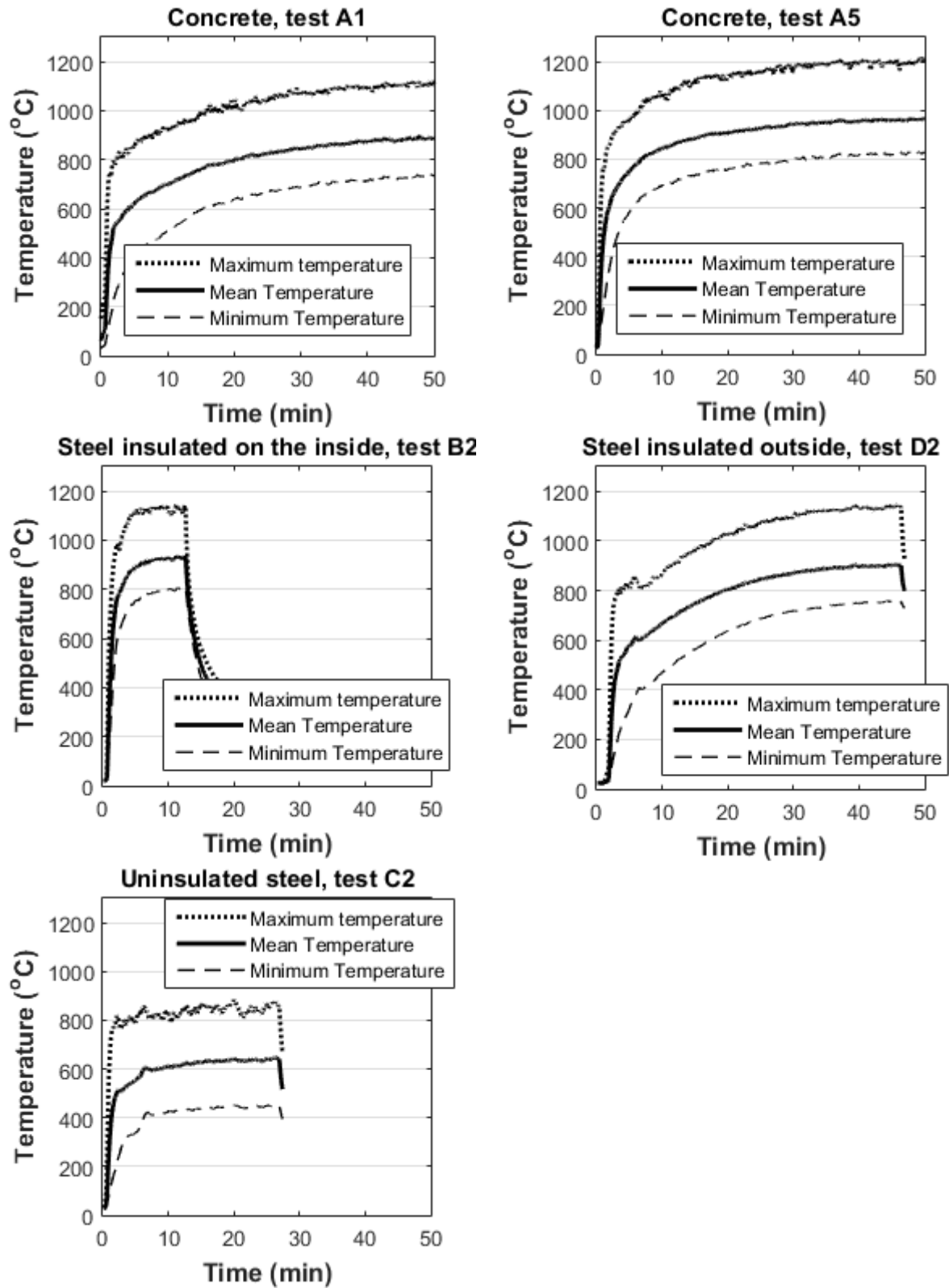
Figure 11. Experimental results of the light weight concrete tests: A1 and A5; the Insulated steel tests: on the inside -B2 and outside -D2, Uninsulated steel tests – C2. These results show compartment mean, maximum and minimum temperatures measured with PTs.
