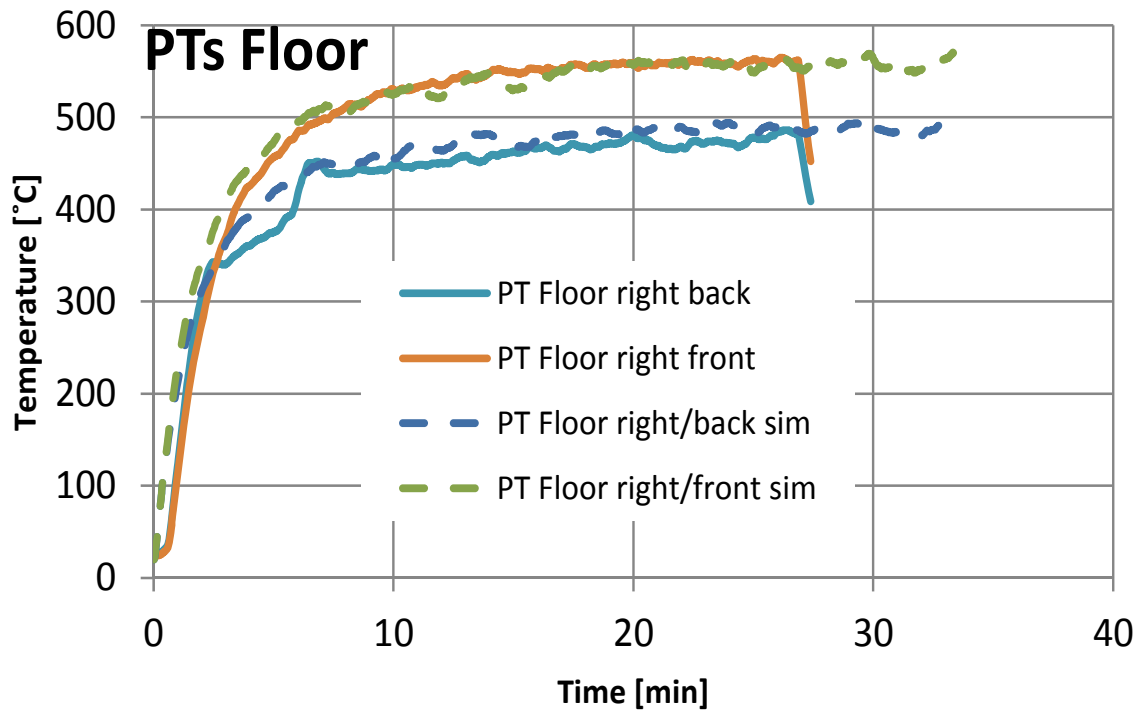
Figure 21 Plate thermometers on the floor.
