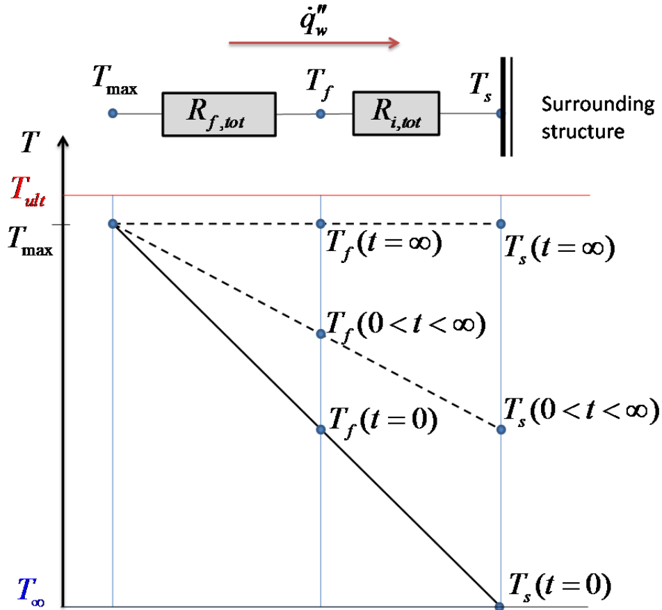
Figure 4. Electrical analogy of the fire model for any structure. The indication of the temperature initially ( t=0 ), after some time ( 0 < t < \infty ) and after a very long time ( t=\infty ).
