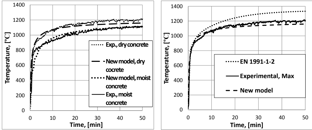
Figure 12. Left: Comparison of calculated and measured temperature. Right: Dry concrete: experimental measured temperature vs. calculated with new model and EN 1991-1-2 ( \Gamma = 15.5 , see Appendix A)
