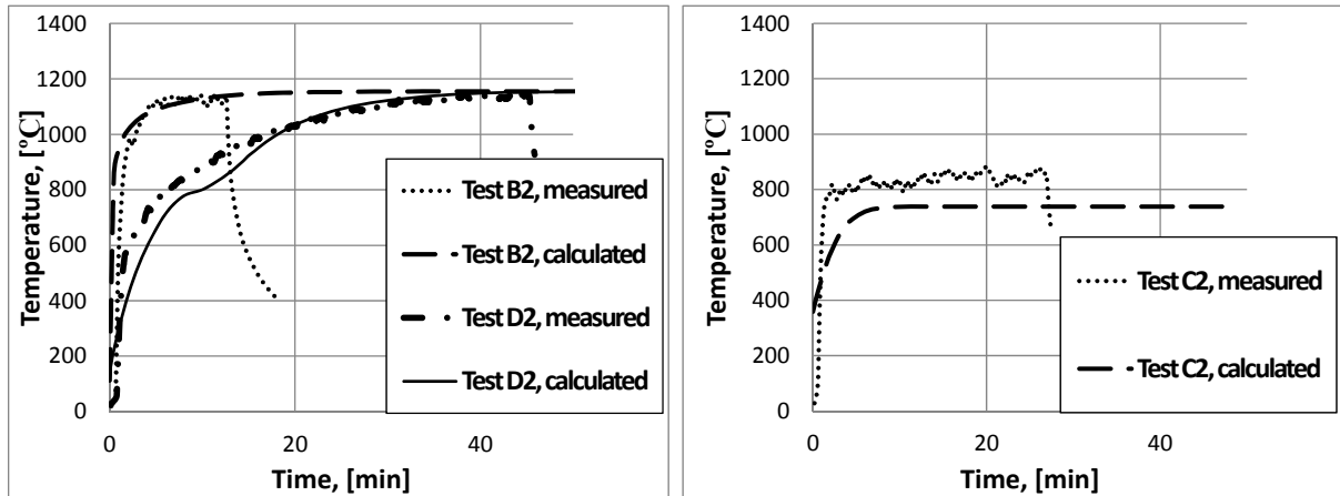
Figure 13. Measured and calculated fire temperatures in fully developed compartment fire in a steel sheet compartment.
