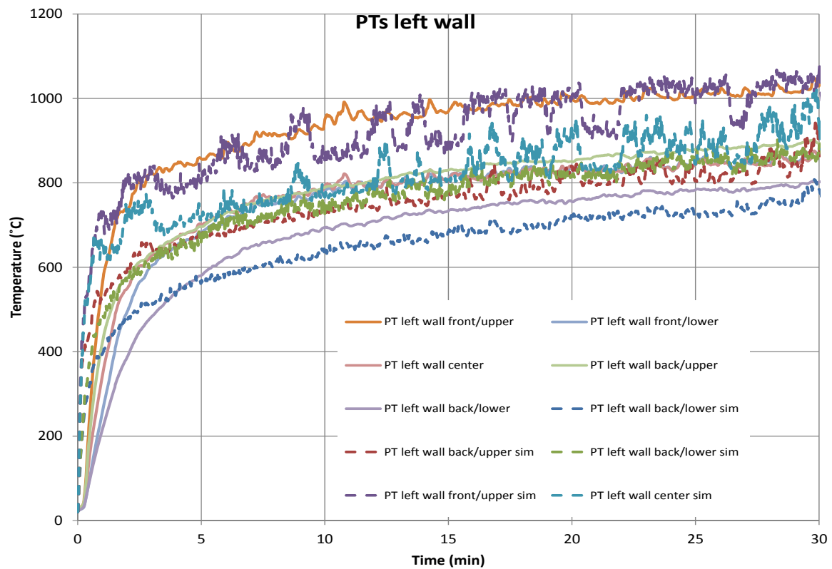
Figure 18 Plate thermometers on the left wall.
