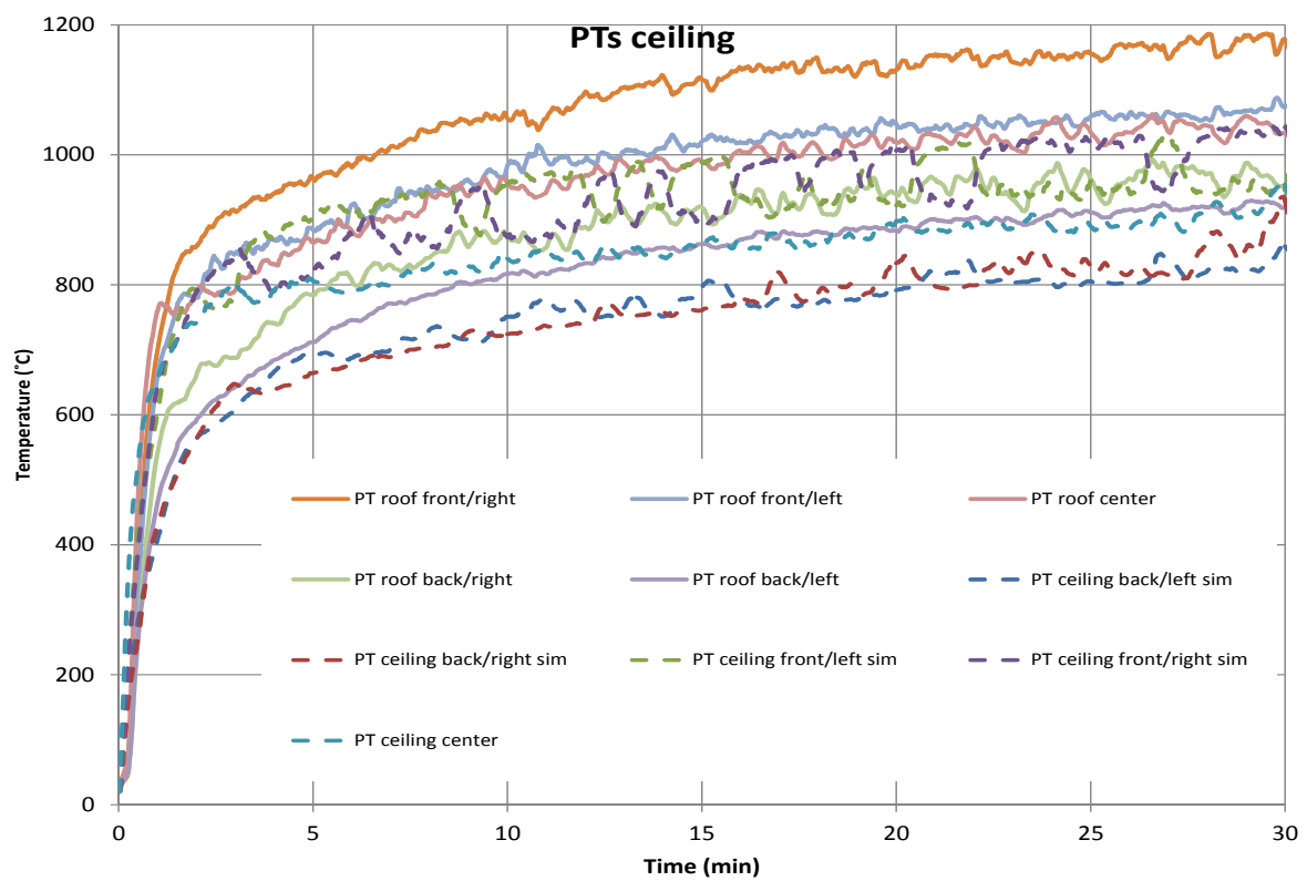
Figure 19 Plate thermometers on the ceiling.
