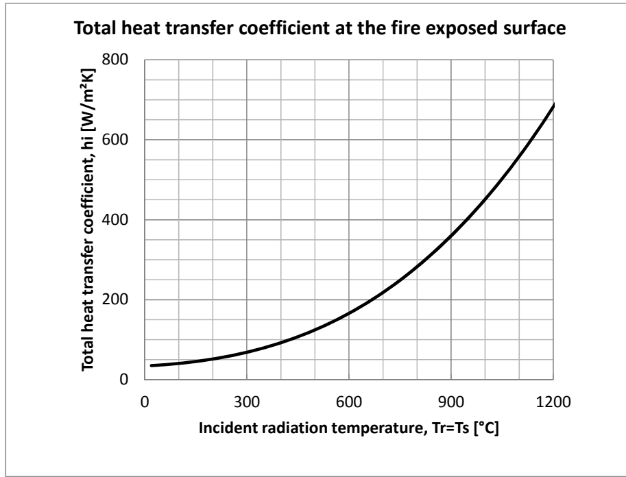
Figure 24. Heat transfer coefficient for the fire exposed surface
