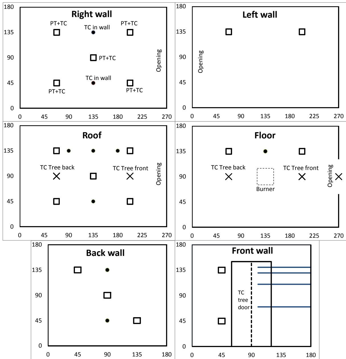
Figure 9 The instrumentation at the inside of the enclosure for test series C and D. The distances are in cm. All squares are PT only unless stated otherwise. All black points are steel temperature measurements. The tubes in the door opening measures CO, CO2 and O 2 gas concentrations at heights 100, 200 and 800 mm from the top of the door opening
