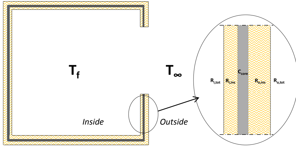
Figure 6 A fire compartment surrounded by a structure with its heat capacity C_{core} assumed concentrated/lumped to a metal core. Thermal resistances of insulation materials R_i and R_o are assumed on the fire inside and outside, respectively.
