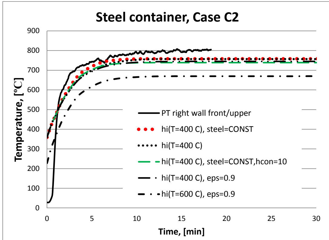
Figure 29. Comparison of calculated temperatures with measured higher temperature during experiments: Experimental measured temperatures with PT vs. calculated ones with Tasef. Non-insulated steel container.
