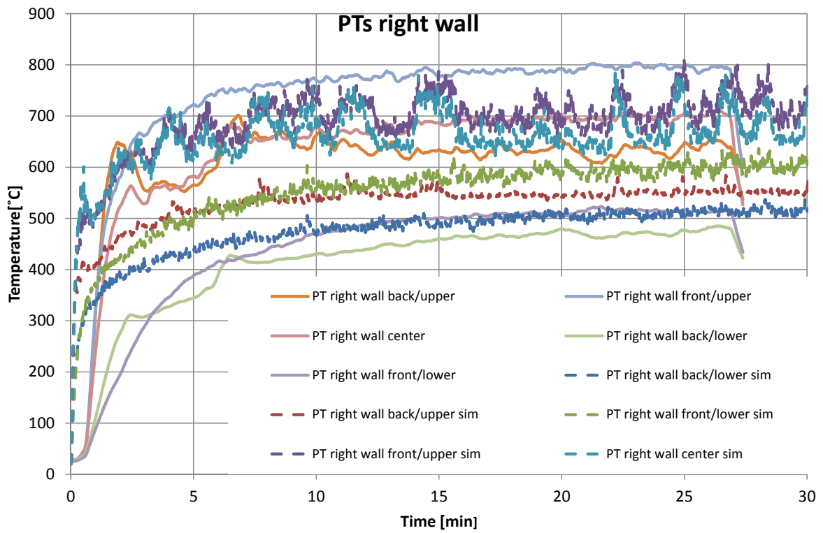
Figure 22 Plate thermometers on the right wall.
