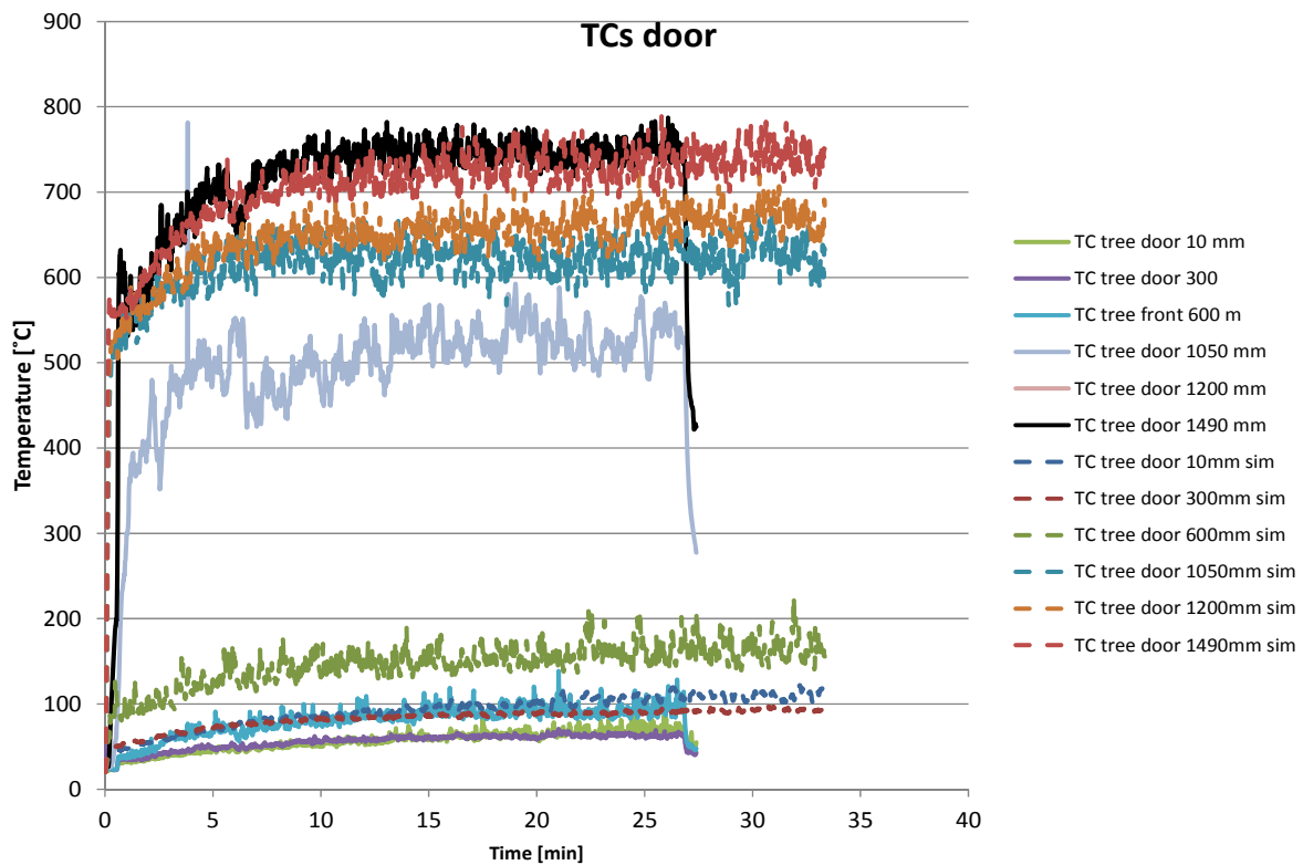
Figure 20 TCs in the door
