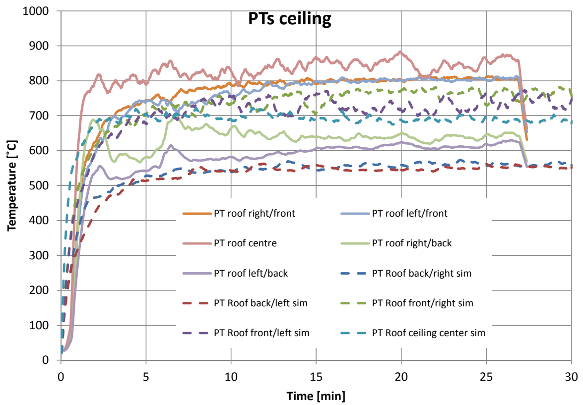
Figure 23 Plate thermometers on the ceiling.
