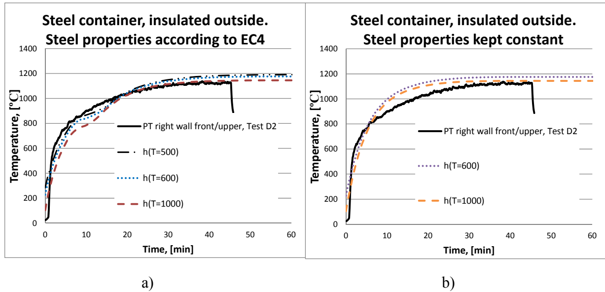
Figure 30. Comparison of calculated temperatures with measured higher temperature during experiments: Experimental measured temperatures with PT vs. calculated ones with Tasef. Insulated outside steel container.
