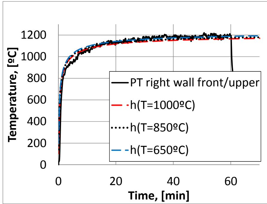
Figure 26. Comparison of calculated temperatures with measured higher temperature during experiments – Case A5.
