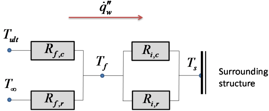
Figure 3. Electric circuit analogy model of a fire compartment boundary according to the new model.
