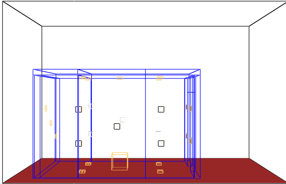
Figure 14 The physical geometry used in the simulations including the placement of the burner and the plate thermometers
