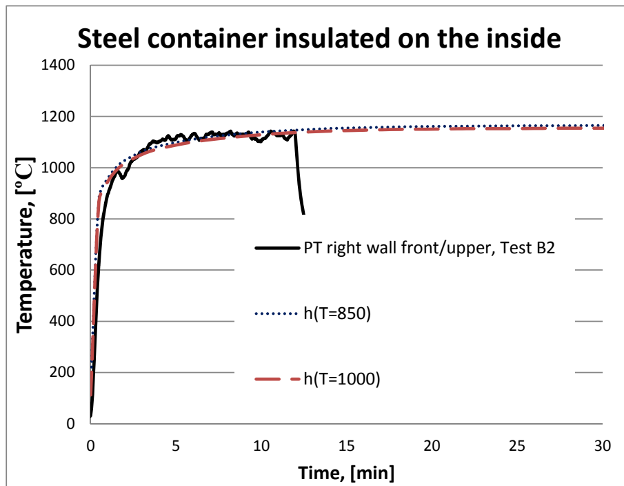
Figure 28. Comparison of calculated temperatures with measured higher temperature during experiments: Experimental measured temperatures with PT vs. calculated ones with Tasef. Insulated on the inside steel container
