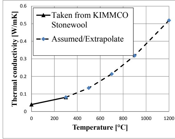
Figure 10 Thermal conductivity of the stone wool used for the FE-modeling
