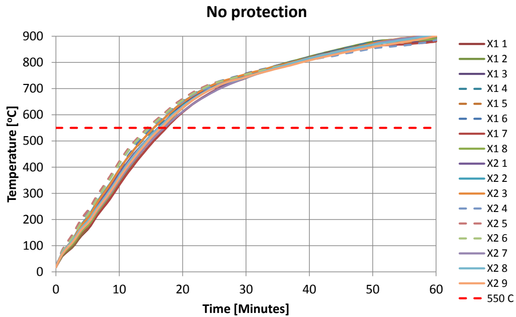
Figure 15 Temperatures in unprotected specimens X1 and X2 during furnace testing. The design temperature 550 °C is included as a reference. Measurements on the bottom side of the specimen are marked with dashed lines.
