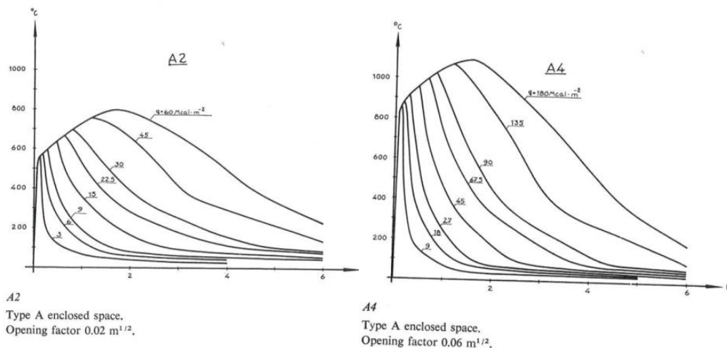
Figure 4 Examples of the “Swedish curves”. Calculated time-temperatures for a range of fuel-load densities, opening factors and enclosure types (Magnusson and Thelandersson, 1970). The left set of curves with opening factor 0.02 \text{ m}^{0.5} rise slower than the standard fire curve and the right set of curves corresponding to opening factor 0.06 \text{ m}^{0.5} rise faster than the standard fire curve.
