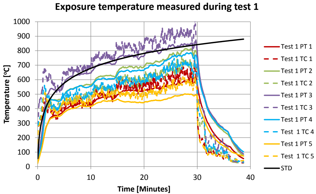
Figure 54 Exposure temperatures during test 1. Plate thermometers and 1 mm shielded thermocouples.
