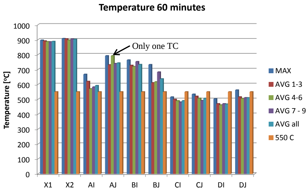
Figure 20 Maximum and average temperatures in all specimens after 60 minutes of standard fire exposure. Thermocouples 4-6 are on the bottom whereas 1-3 and 7-9 are on the horizontal part of the specimens.
