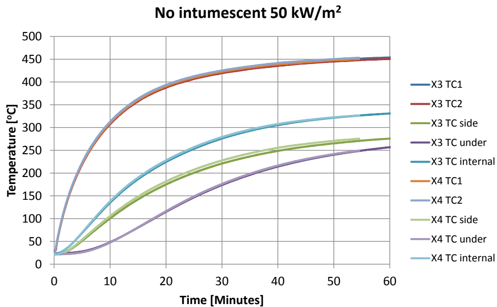
Figure 45 Cone calorimeter tests on steel without intumescent paint, 50 kW/m 2 exposure.
