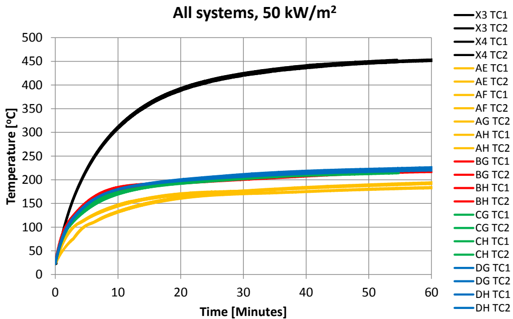
Figure 10 Cone calorimeter tests during incident heat flux 50 kW/m 2 . Shown in the graph are steel temperatures on the heat exposed surface. All measurements can be seen in Appendix A.
