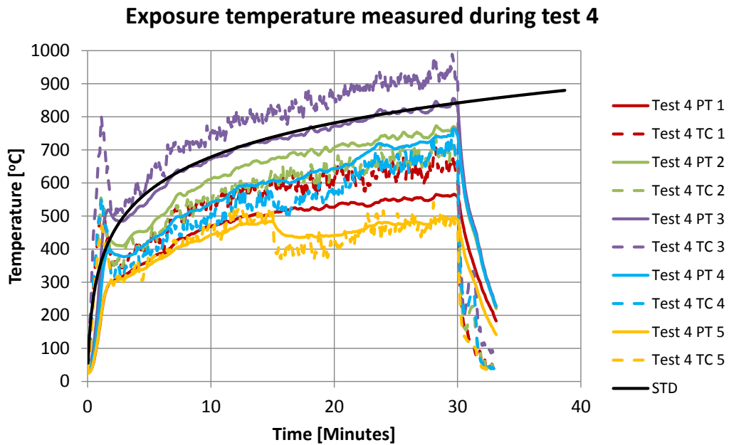
Figure 57 Exposure temperatures during test 4. Plate thermometers and 1 mm shielded thermocouples.
