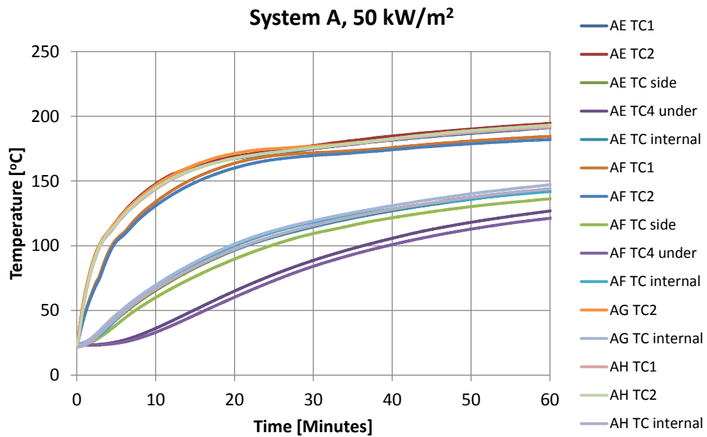
Figure 47 Cone calorimeter tests on steel with intumescent paint system A, 50 kW/m 2 exposure.
