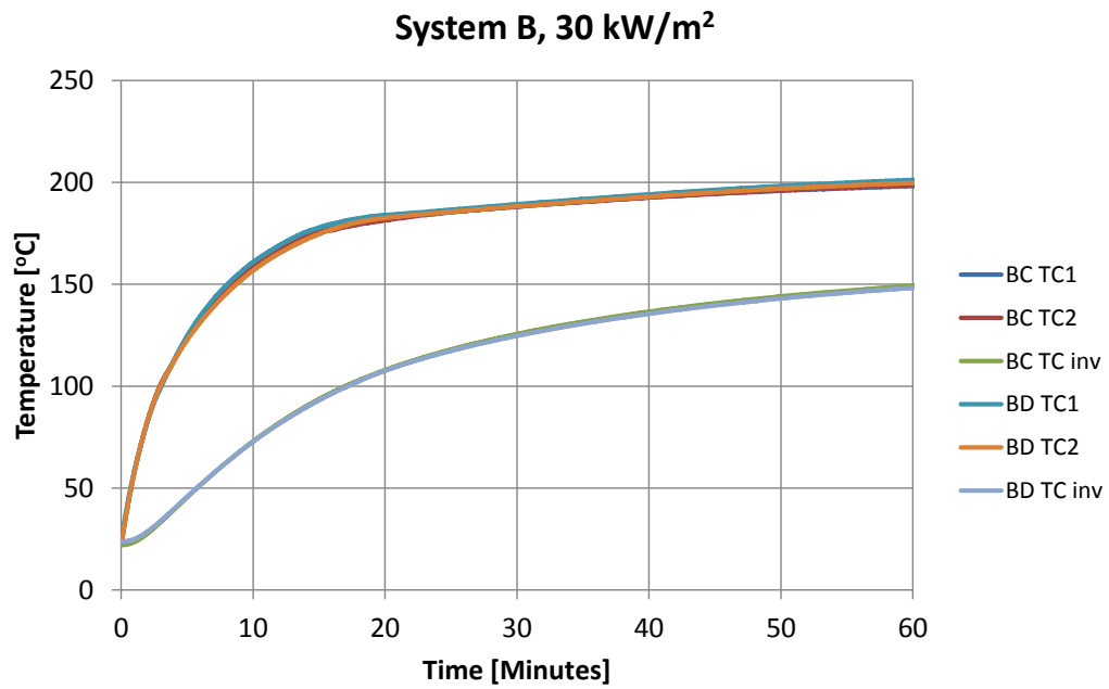
Figure 48 Cone calorimeter tests on steel with intumescent paint system B, 30 kW/m 2 exposure.
