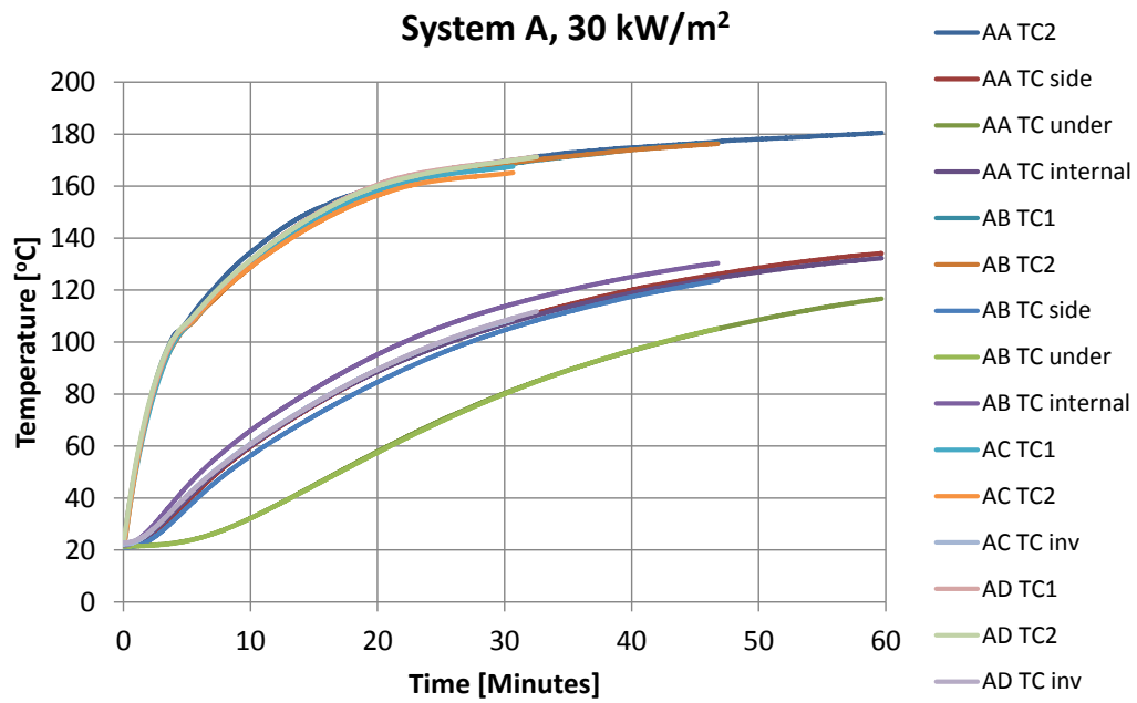
Figure 46 Cone calorimeter tests on steel with intumescent paint system A, 30 kW/m 2 exposure.
