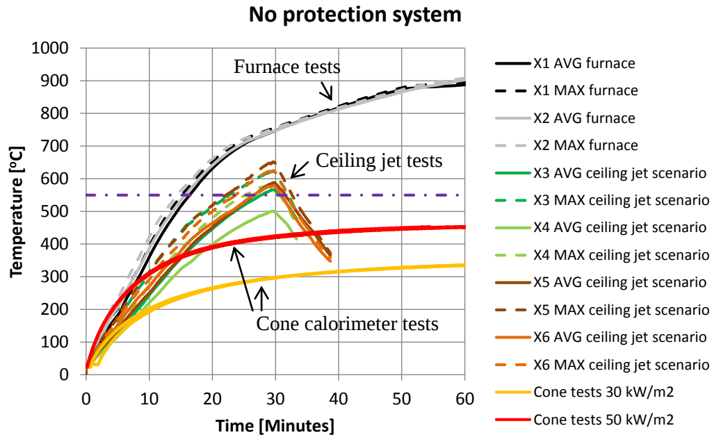
Figure 39 Summary of temperature development in reference specimens during furnace, ceiling jet, fire plume and cone calorimeter tests. The design temperature 550 °C is marked with a horizontal line. Fire plume exposure of unprotected steel was not included in the study.
