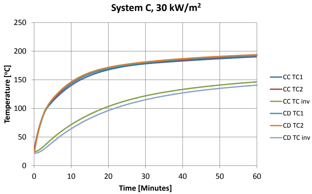
Figure 50 Cone calorimeter tests on steel with intumescent paint system C, 30 kW/m 2 exposure.
