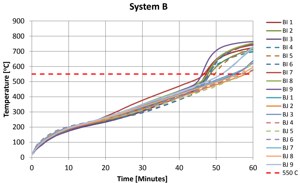
Figure 17 Temperatures in system B specimens during furnace testing. The design temperature 550 °C is included as a reference. Measurements on the underside of the specimen is marked with dashed lines.
