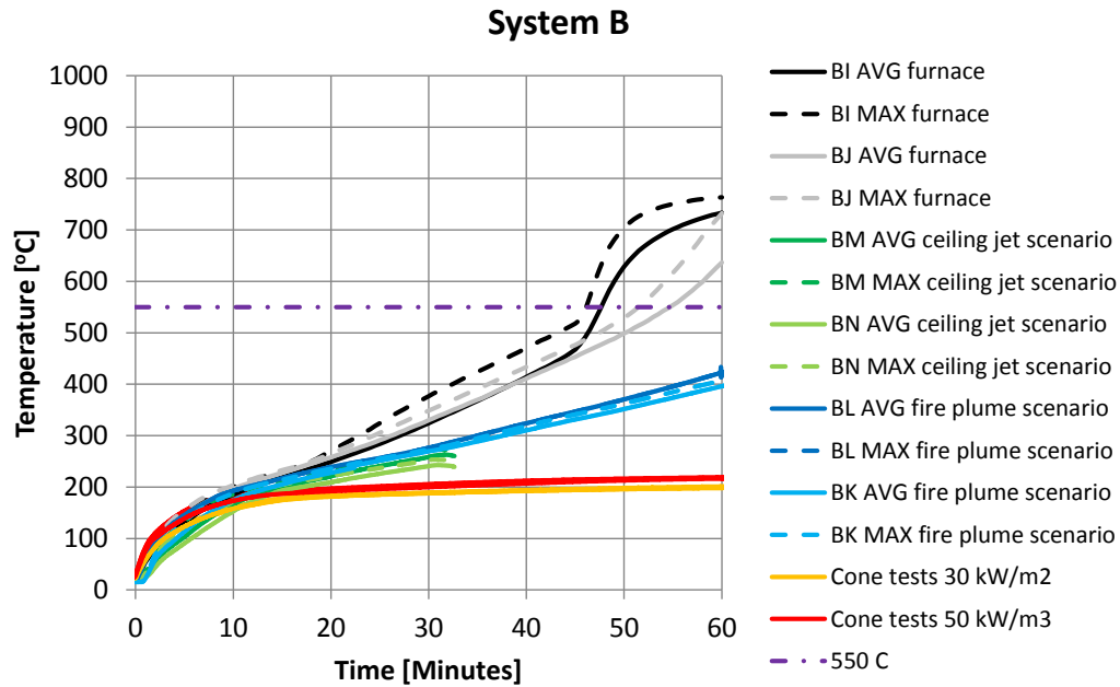
Figure 41 Summary of temperature development in specimens protected with system B during furnace, ceiling jet, fire plume and cone calorimeter tests. The design temperature 550 °C is marked with a horizontal line.
