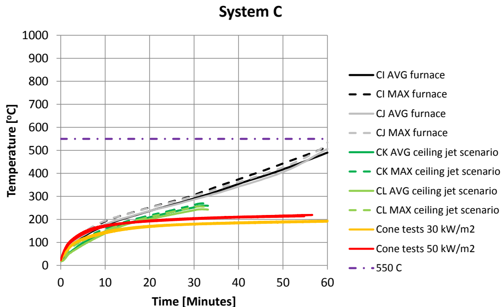
Figure 42 Summary of temperature development in specimens protected with system C during furnace, ceiling jet, fire plume and cone calorimeter tests. The design temperature 550 °C is marked with a horizontal line. Fire plume exposure of system C was not included in the study.
