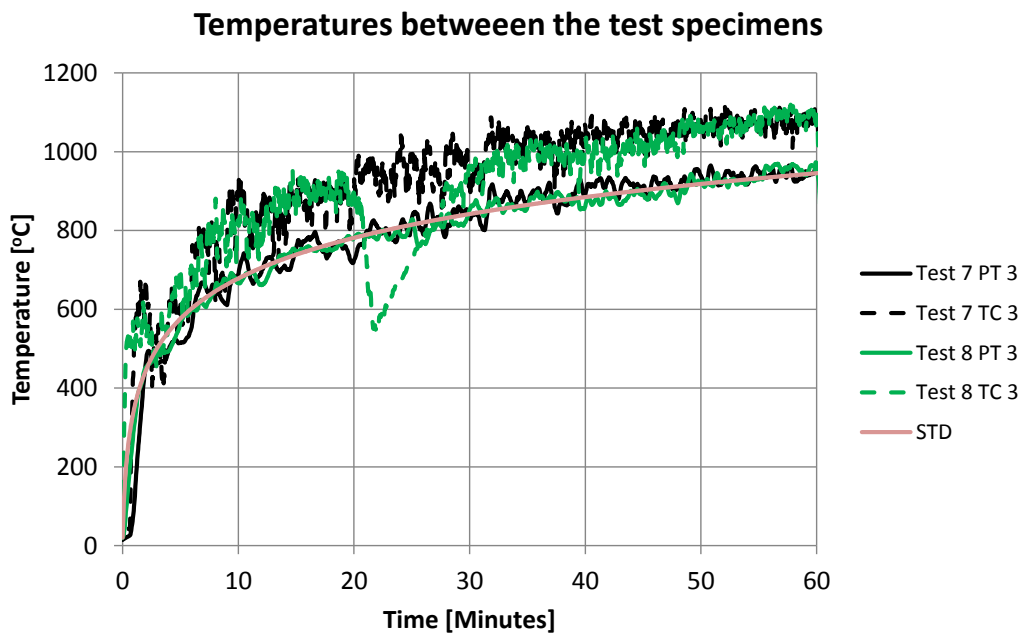
Figure 36 Temperatures measured between the test specimens in the fire plume. The dip in temperature for TC 3 in test 8 was due to large chunks of intumescent paint from the type A system resting against it.
