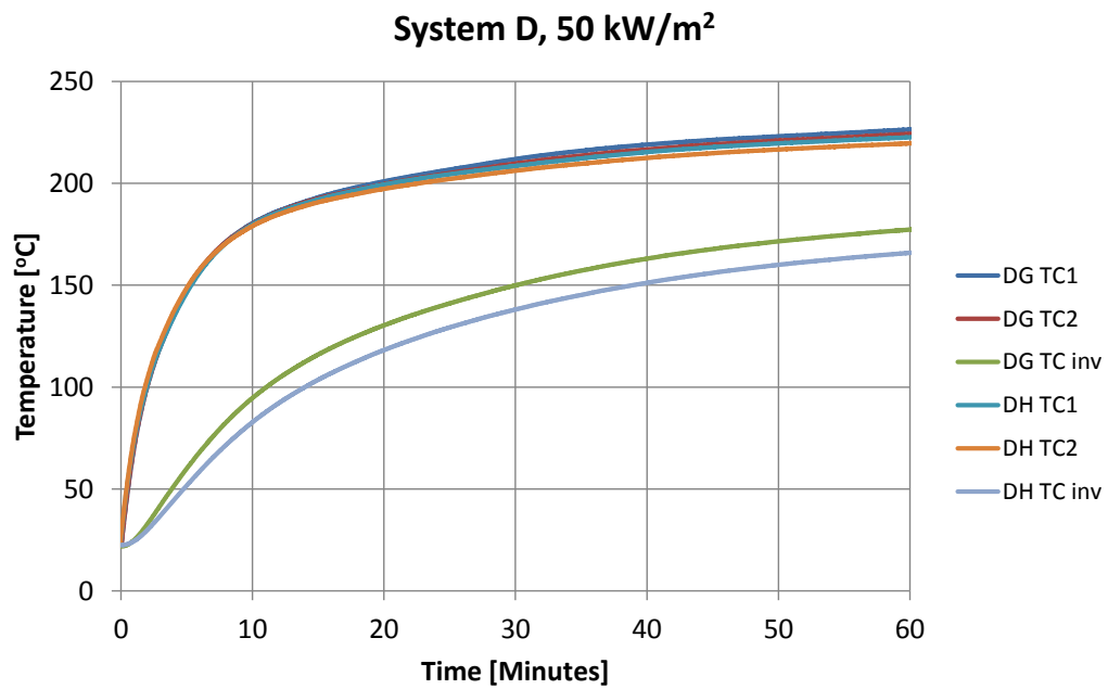
Figure 53 Cone calorimeter tests on steel with intumescent paint system D, 50 kW/m 2 exposure.
