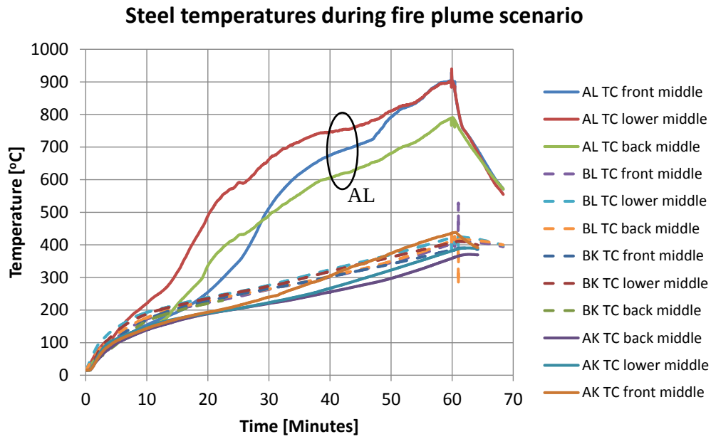
Figure 38 Temperatures measured in the steel sections during fire plume scenario. Specimen AL and BL were tested during test 8 and specimen BK and AK were tested during test number 7. The exposure data during test 7 and 8 can be seen in Figure 36.
