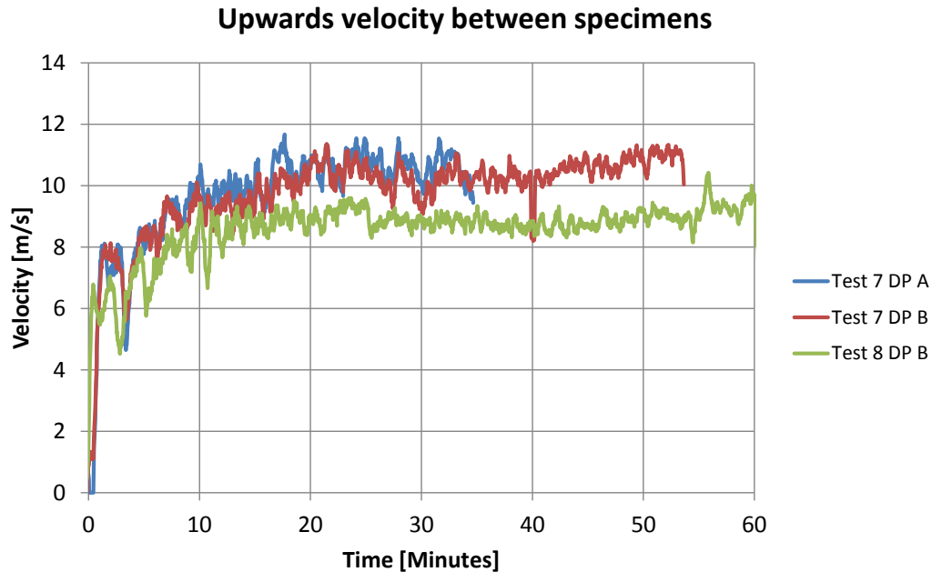
Figure 37 Estimated upwards velocities between the specimens during the fire plume scenario. DP in figure means Differential Pressure probe. The calculation procedure for calculation of velocities based on differential pressure probe measurement can be found in Chapter 2.3.3.
