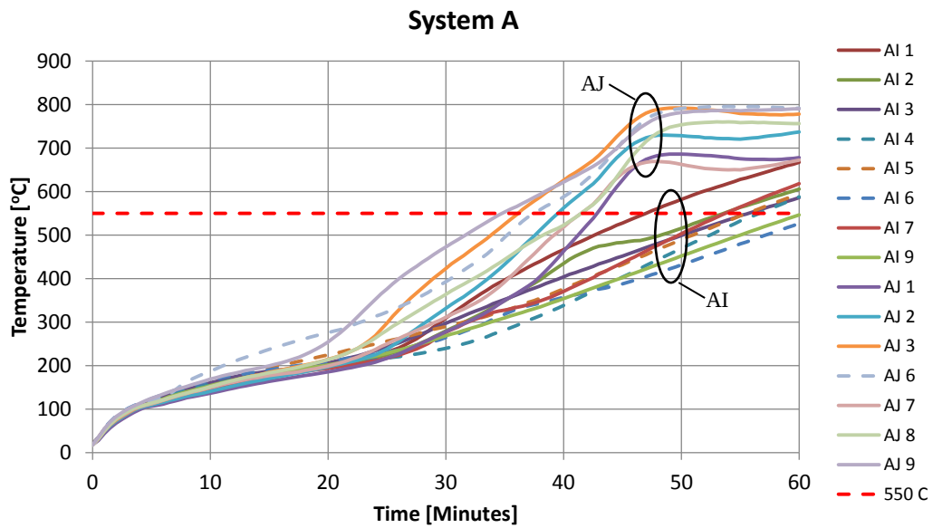
Figure 16 Temperatures in system A specimens during furnace testing. The design temperature 550 °C is included as a reference. Measurements on the underside of the specimen is marked with dashed lines.
