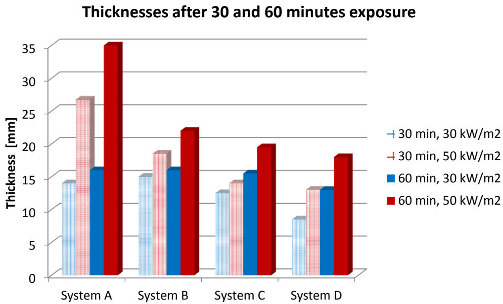
Figure 12 Thickness after 30 and 60 minutes of exposure for all systems during both radiation levels.
