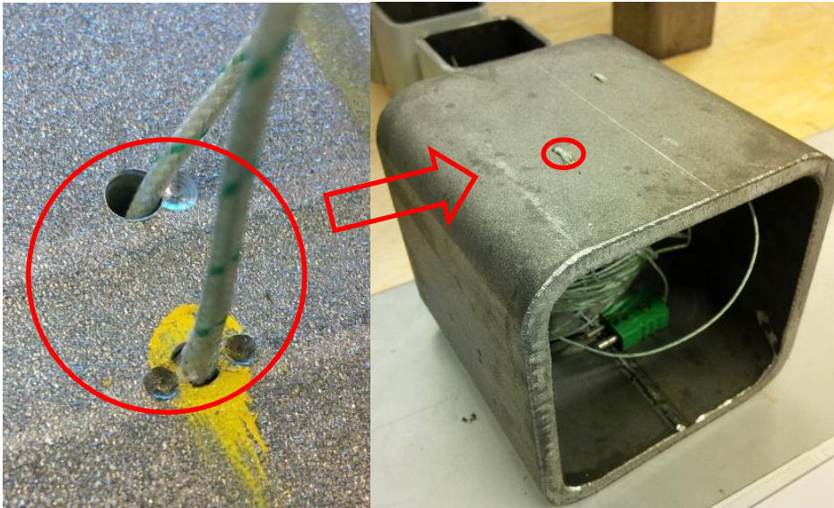
Figure 6 a) Quick tip mounted and TC wire routed through the specimen surface. After stretching the TC wire mounting is shown in figure b. b) Test specimen for cone calorimeter test with two TCs. Photo: Ulla Eidissen Jensen
