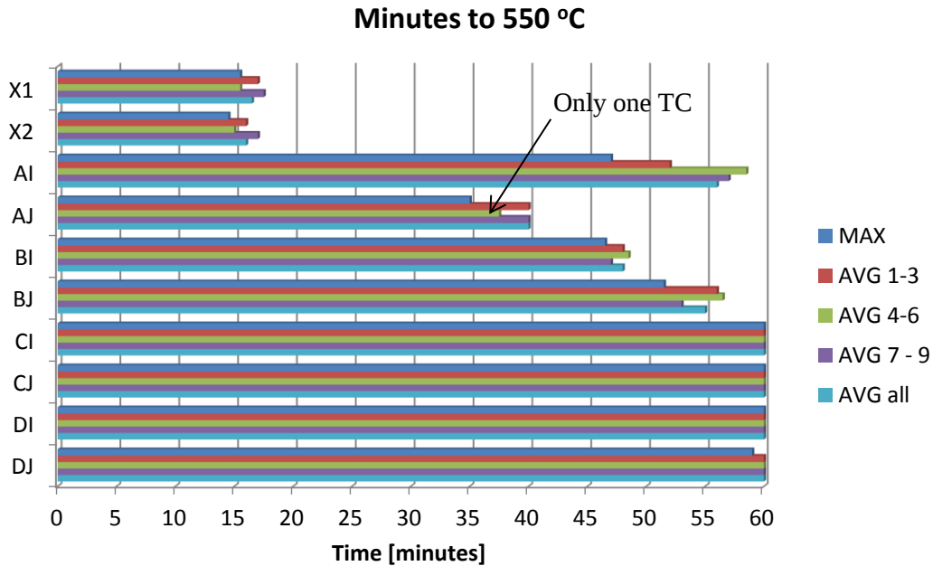
Figure 21 Time to reach the design temperature 550 °C during standard fire exposure. Thermocouples 4-6 are on the bottom, horizontal part of the specimens. Specimen CI, CJ, DI and average temperatures in specimens DJ did not reach 550 °C during 60 minutes.
