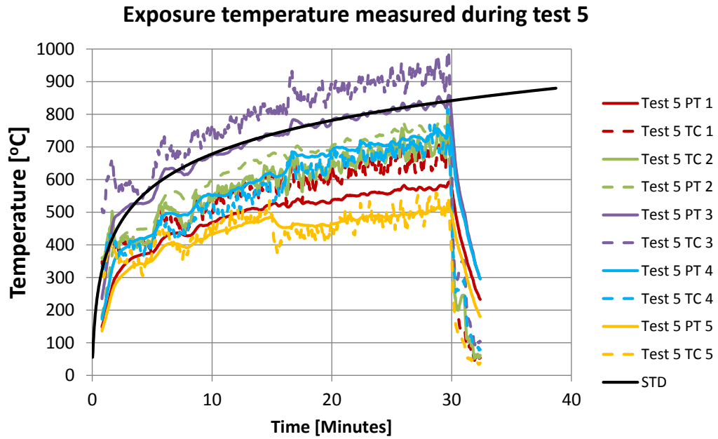
Figure 58 Exposure temperatures during test 5. Plate thermometers and 1 mm shielded thermocouples.
