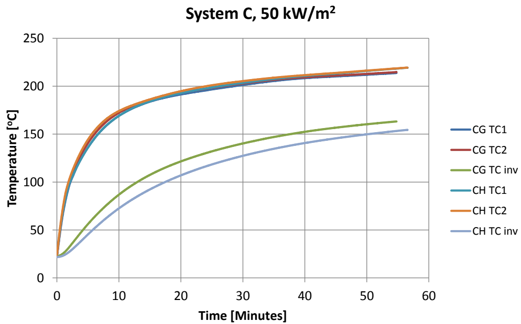
Figure 51 Cone calorimeter tests on steel with intumescent paint system C, 50 kW/m 2 exposure.
