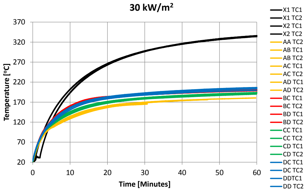
Figure 9 Cone calorimeter tests with incident heat flux 30 \text{ kW/m}^2 . Shown in the graph are steel temperatures on the heat exposed surface. All measurements can be seen in Appendix A.
