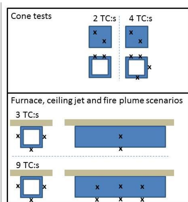
Figure 7 Thermocouple (TC) placement. In the cone tests the two upper TCs were placed in the centre of the quadrants of the surface.
