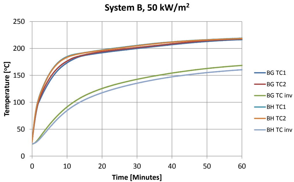
Figure 49 Cone calorimeter tests on steel with intumescent paint system B, 50 kW/m 2 exposure.
