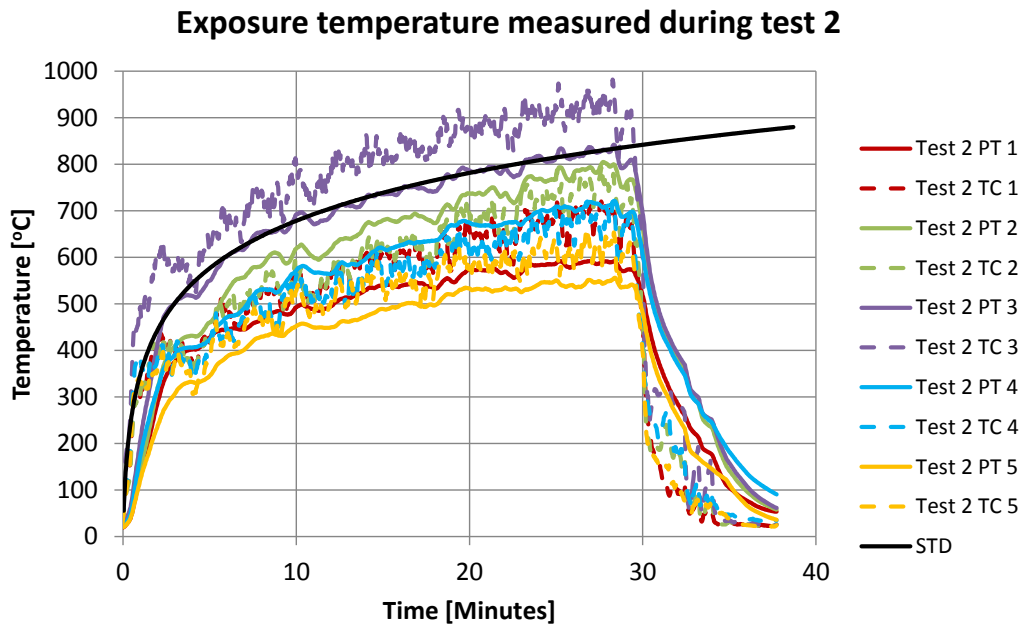
Figure 55 Exposure temperatures during test 2. Plate thermometers and 1 mm shielded thermocouples.
