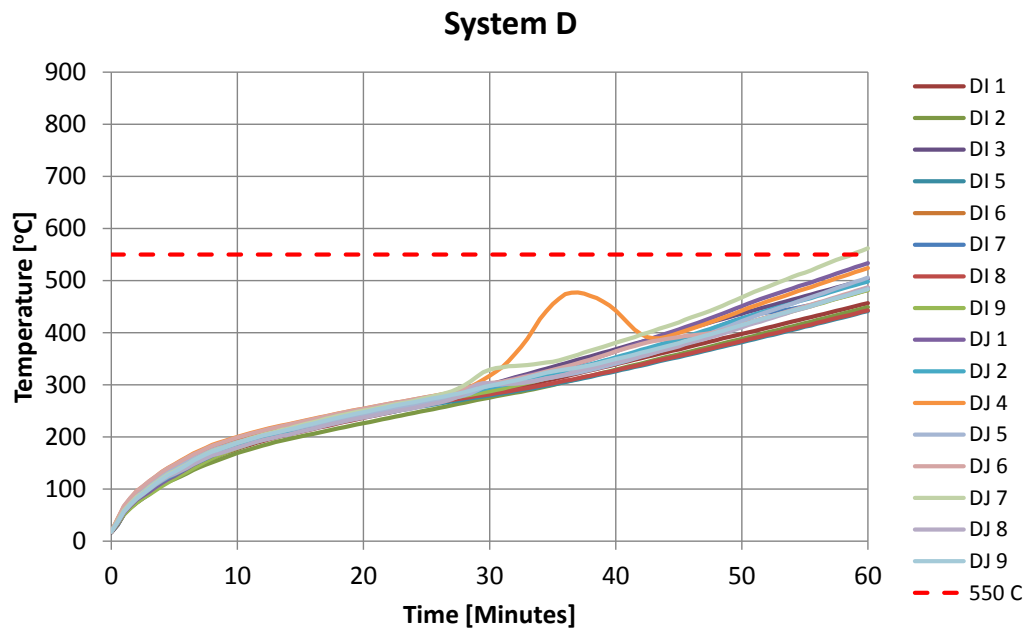
Figure 19 Temperatures in system D specimens during furnace testing. The design temperature 550 °C is included as a reference.
