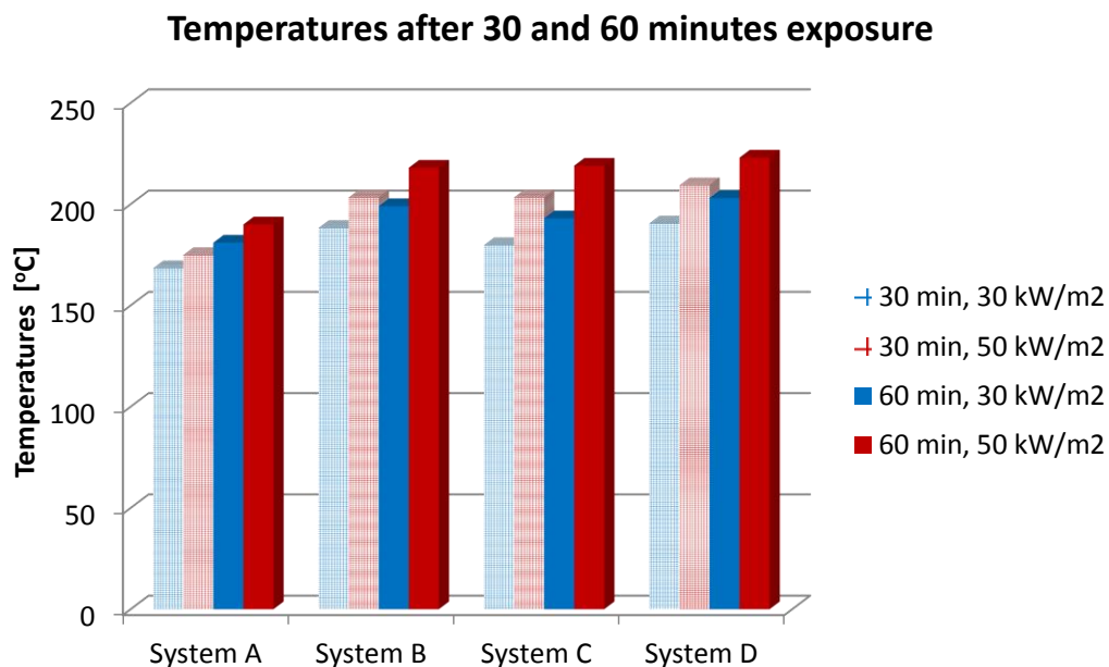
Figure 11 Temperatures after 30 and 60 minutes of exposure for all systems during both radiation levels.
