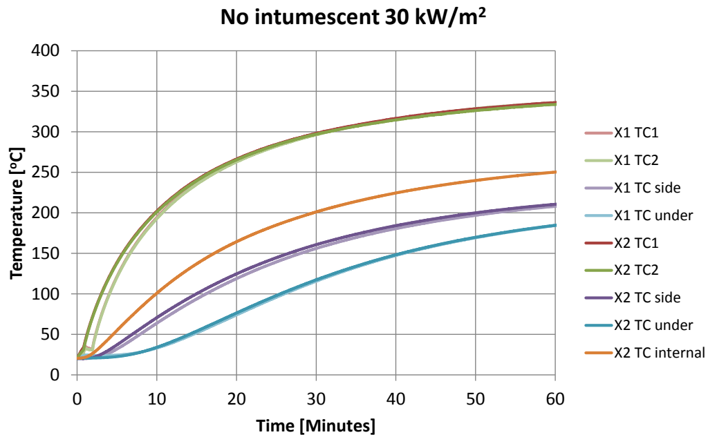
Figure 44 Cone calorimeter tests on steel without intumescent paint, 30 kW/m 2 exposure.
