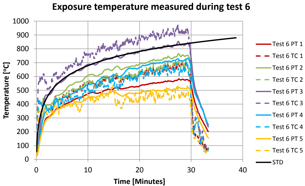
Figure 59 Exposure temperatures during test 6. Plate thermometers and 1 mm shielded thermocouples.
