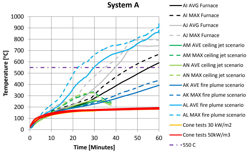
Figure 40 Summary of temperature development in specimens protected with system A during furnace, ceiling jet, fire plume and cone calorimeter tests. The design temperature 550 °C is marked with a horizontal line.
