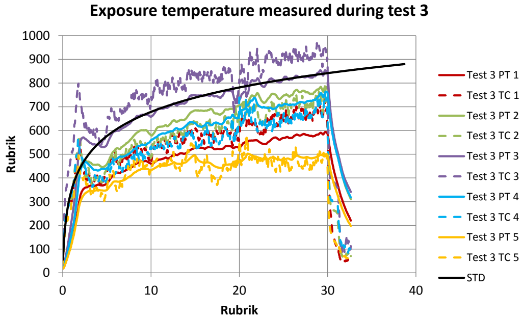
Figure 56 Exposure temperatures during test 3. Plate thermometers and 1 mm shielded thermocouples.
