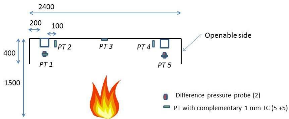
Figure 23 Cross section of test setup for testing two specimens with square cross section in the ceiling jet scenario. The depth of the rig was 900 mm. Instrumentation included plate thermometers (PT), 1 mm shielded thermocouples and differential pressure probes.
