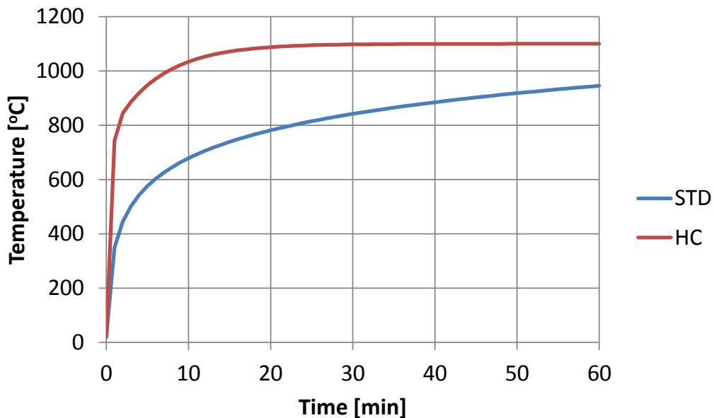
Figure 2 The standard fire exposure also called the “cellulosic” fire and the hydrocarbon fire exposure according to EN 1363:2012.
