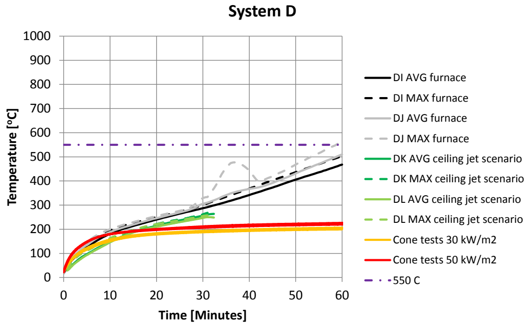
Figure 43 Summary of temperature development in specimens protected with system D during furnace, ceiling jet, fire plume and cone calorimeter tests. The design temperature 550 °C is marked with a horizontal line. Fire plume exposure of system D was not included in the study.
