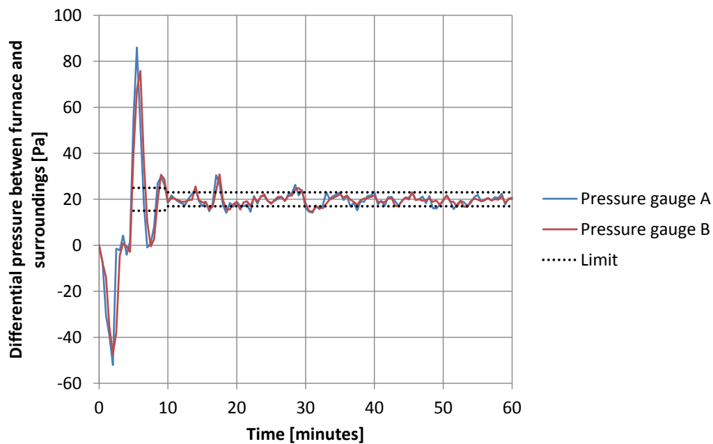
Figure 14 Pressure difference between furnace and surroundings on the height 100 mm beneath the furnace roof as measured with two different gauges. The pressure was outside the limits stated in the standard during the time 5-10 minutes.
