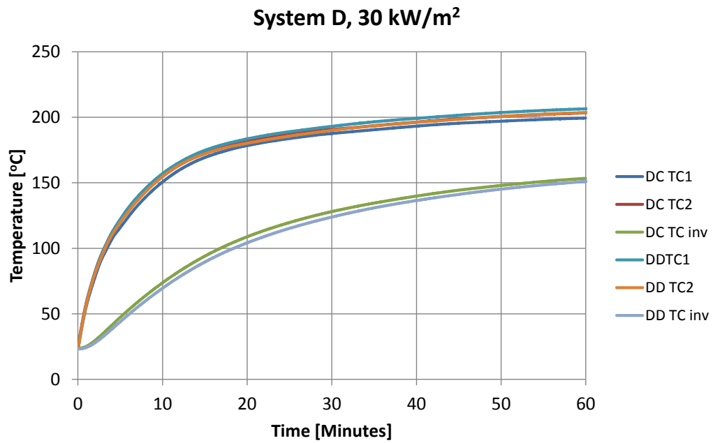
Figure 52 Cone calorimeter tests on steel with intumescent paint system D, 30 kW/m 2 exposure.
