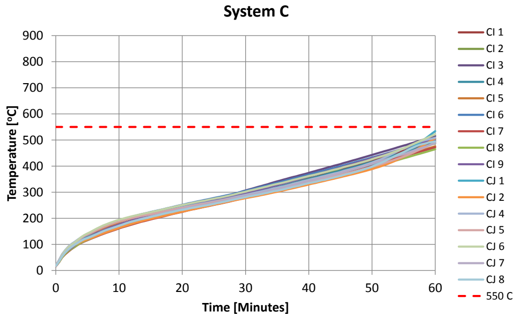
Figure 18 Temperatures in system C specimens during furnace testing. The design temperature 550 °C is included as a reference.
