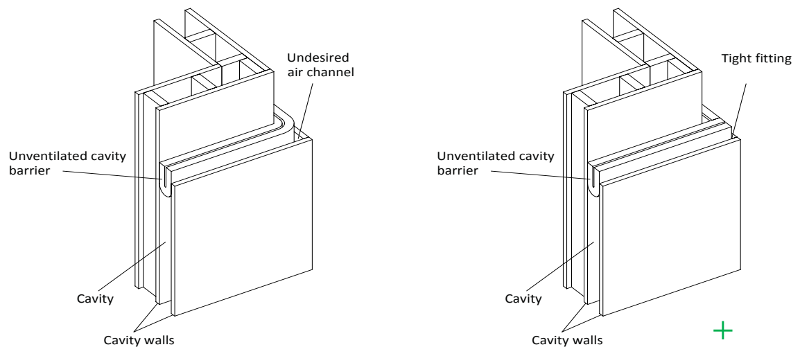
Figure 20 - Possible risk for undesired air channel in the outer corner
