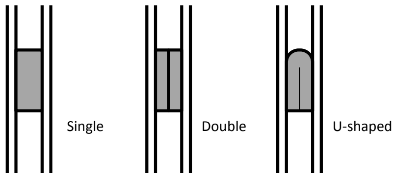
Figure 3 - Single, Double and U-shaped positioning between two cavity walls
