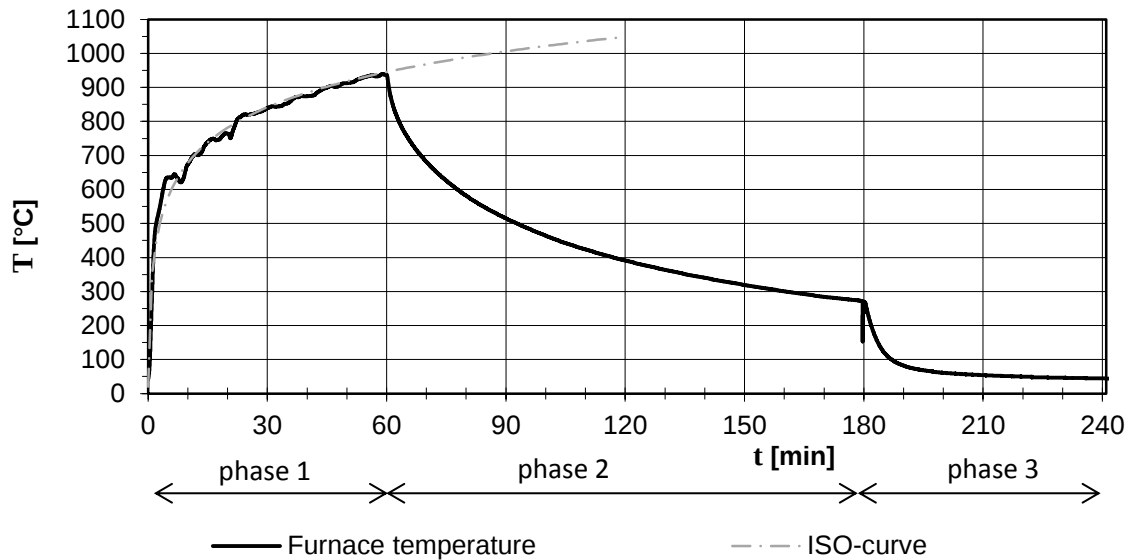
Figure 9 - Average heat exposure measured using two plate thermometers (test 1)
