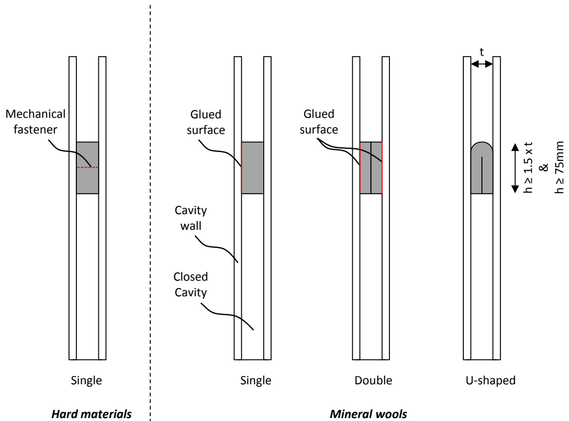
Figure 18 – Cross-sections of single double and U-shaped cavity barriers
