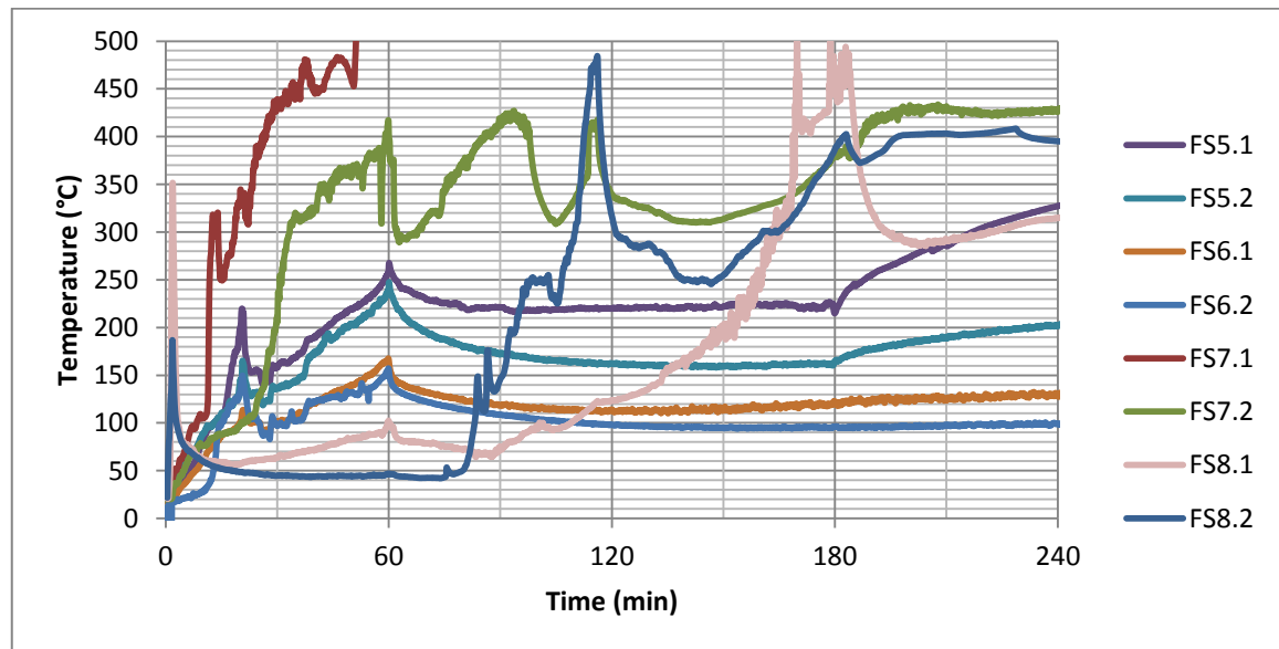
Figure 10 - Temperatures measured in the centre of the cavities
