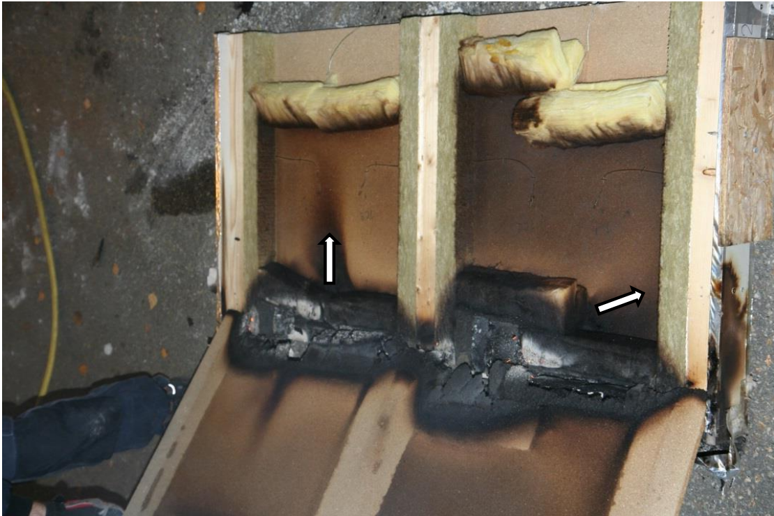
Figure 15 - Inside of the cavities FSJ2.1 (right) and FSJ2.2 (left) after the test
