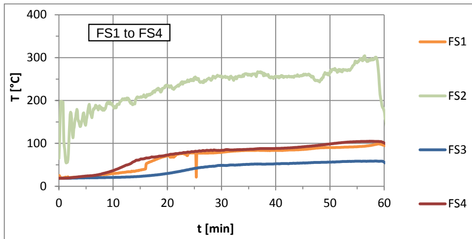
Figure 4: temperatures on the unexposed side of the cavity barriers
