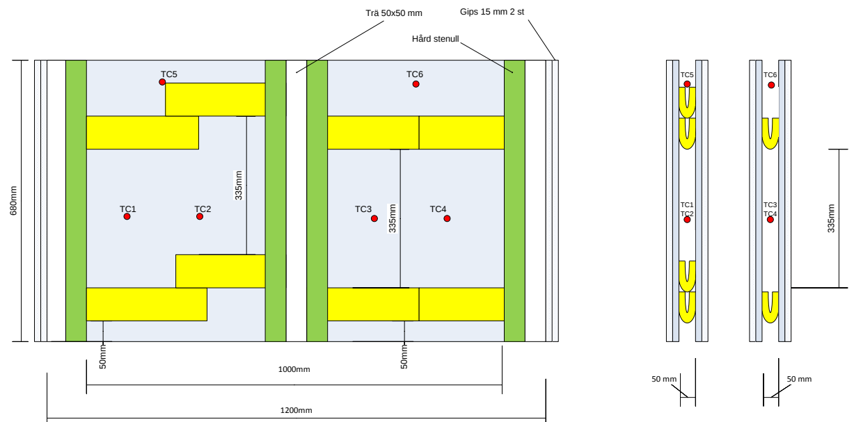
Figure 11 - Cross-sections of specimens with overlapping joints (left) and butt joints (right), exposed from the bottom
