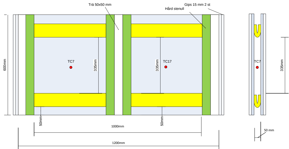
Figure 8 - Cross-sections of specimens of test series 2, exposed from the bottom
