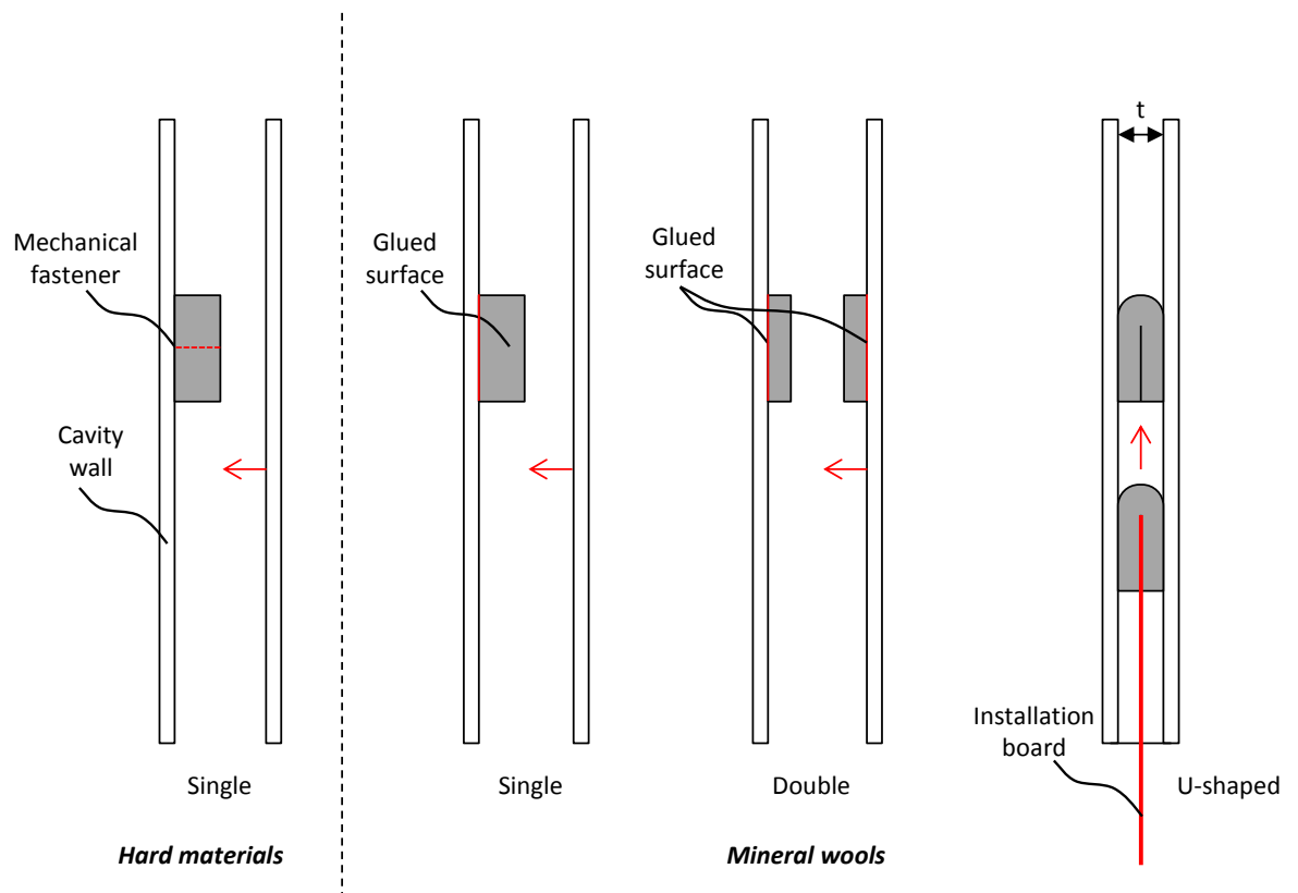
Figure 21 – Schematic drawing of installation
