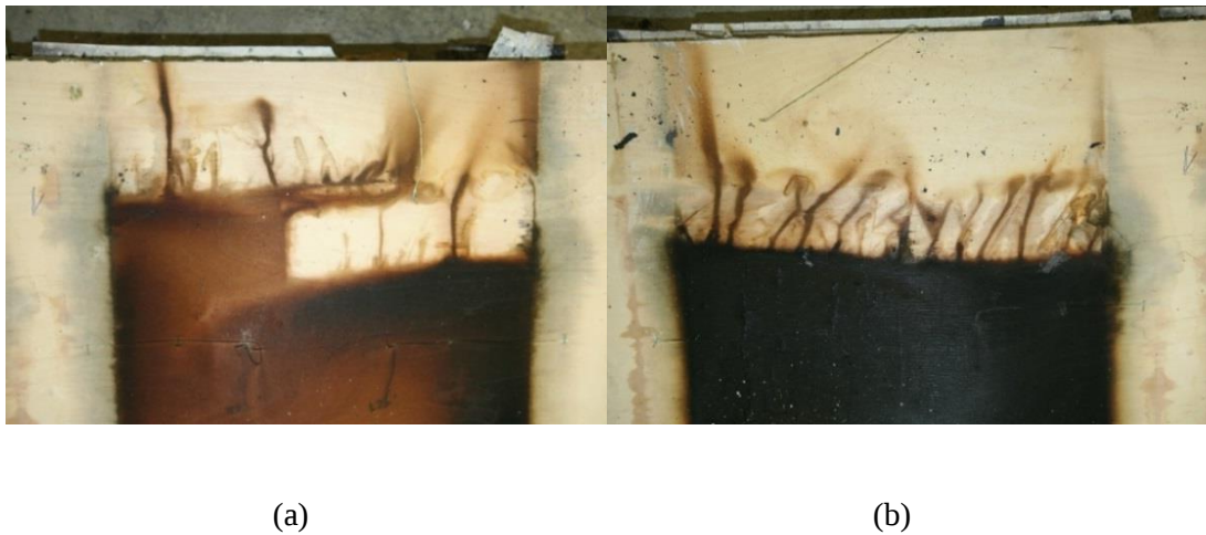
Figure 13 - Cavity walls of FSJ1.1 (a) and FSJ1.2 (b) after the test
