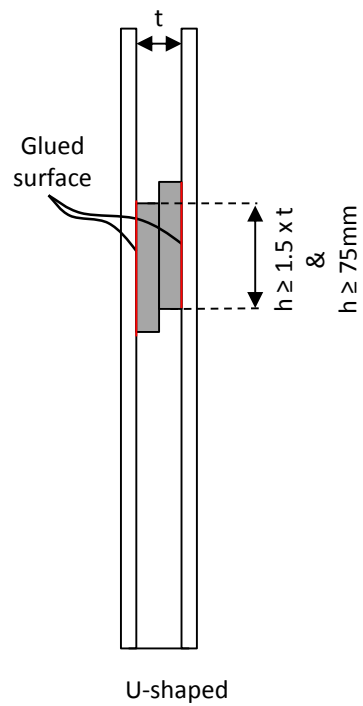
Figure 22 – Allowable geometrical misalignment
