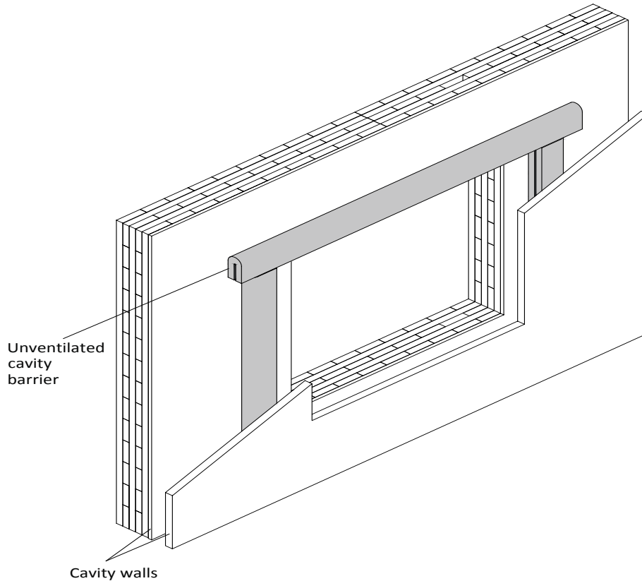
Figure 19 - Prevention from falling of cavity barrier by robust design
