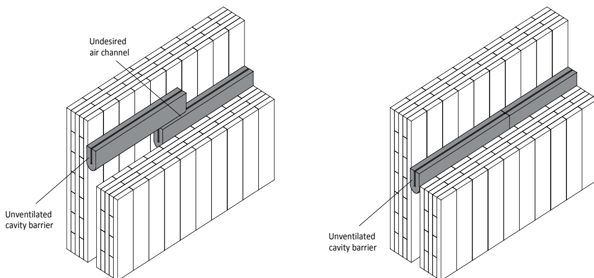
Figure 24 - Possible risk for undesired air channel with overlapped joint
