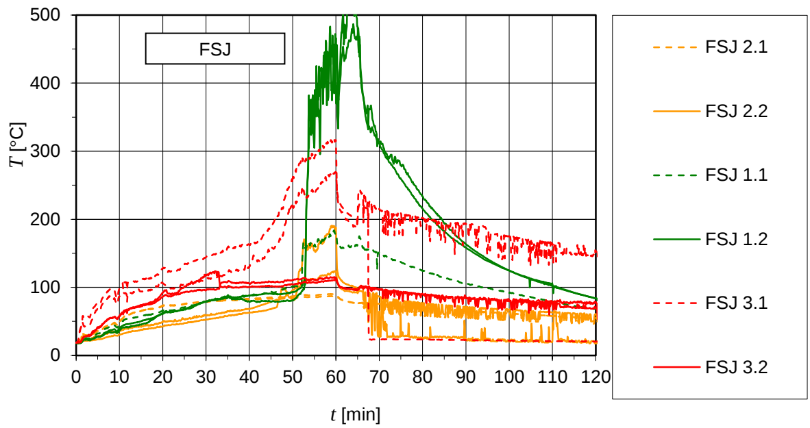
Figure 12 - Temperature measured in the center of the cavities
