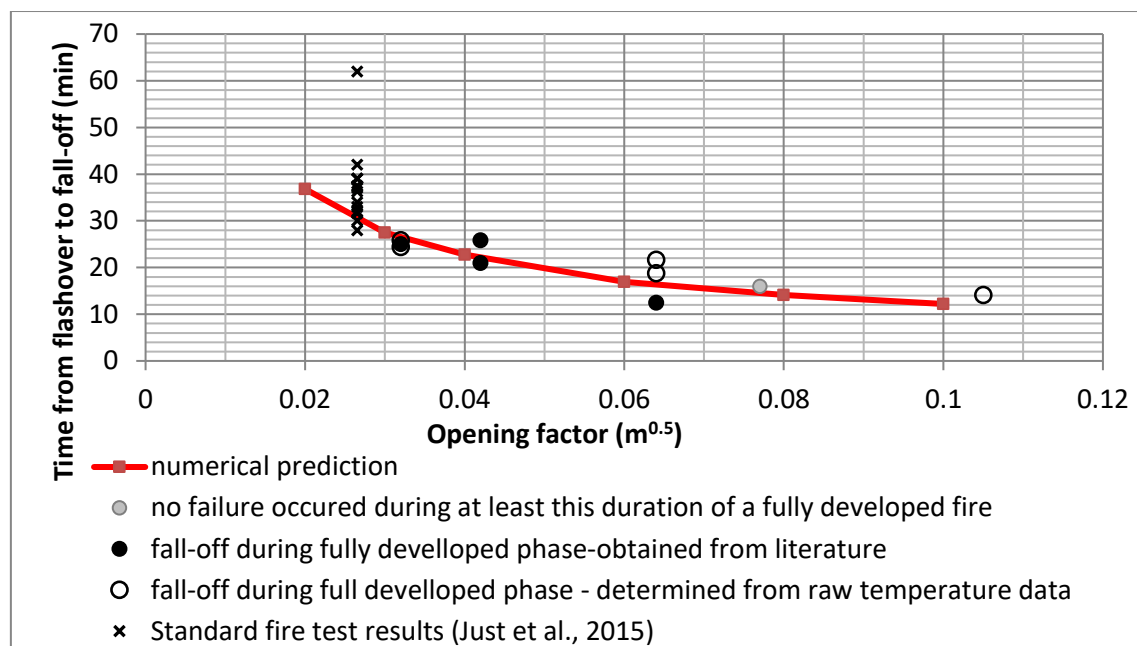
Figure 3: Time from flashover to gypsum fall-off (only fall-off in the fully developed phase is considered)
