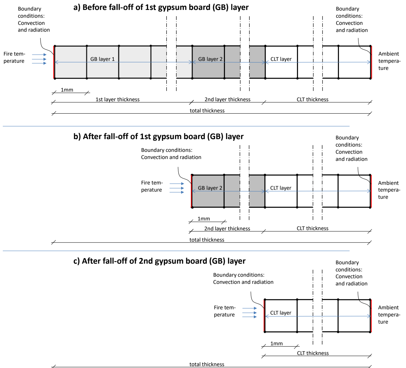
Figure A2: Schematic drawing a finite element model for calculations of temperatures behind gypsum boards.
