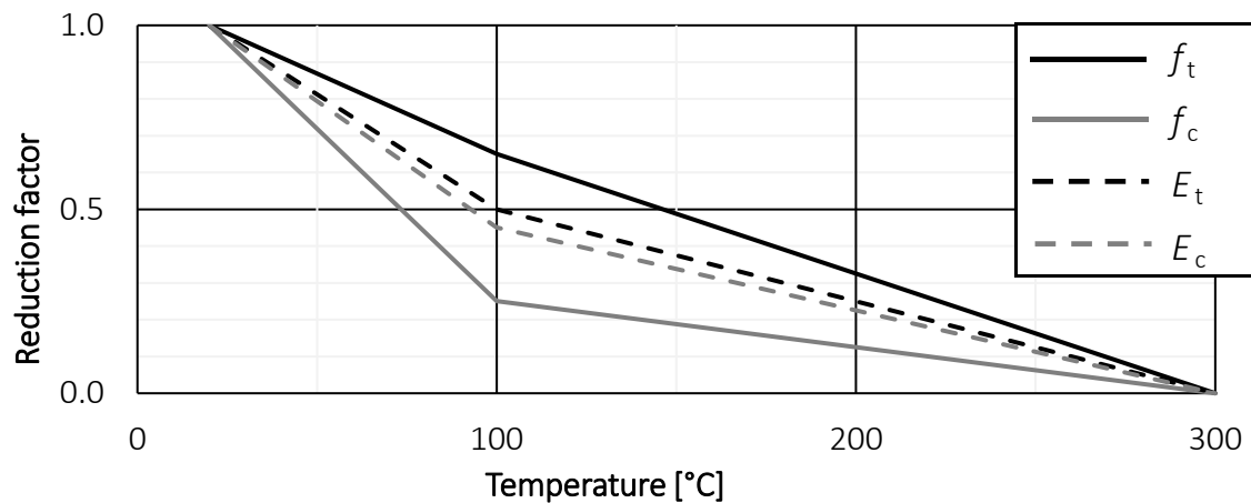
Figure 7: Temperature dependent reduction factors for strength and Young's modulus
