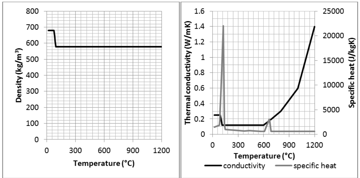
Figure 2: Effective thermal properties for temperature calculations of gypsum board.
