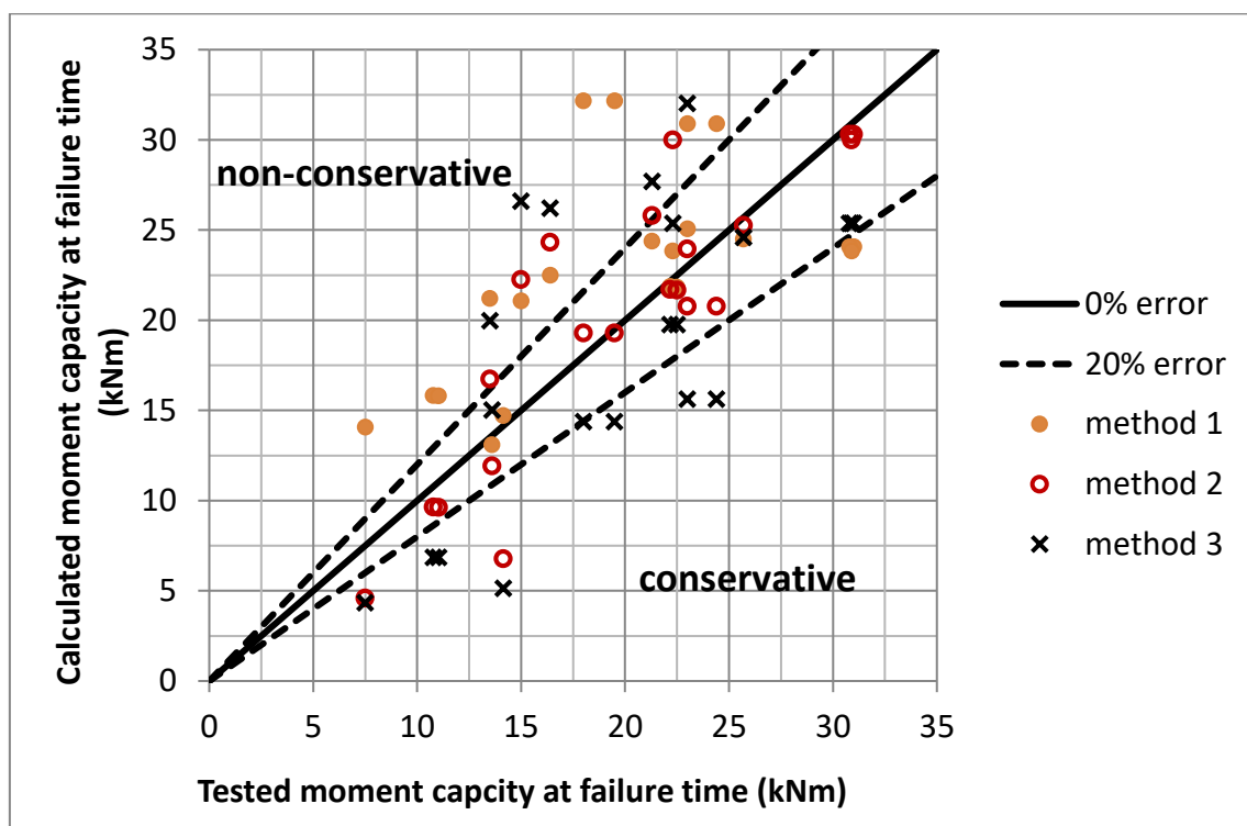
Figure 8: Predicted versus experimental moment capacity at the time of failure of glued laminated timber beams exposed to parametric fires.
