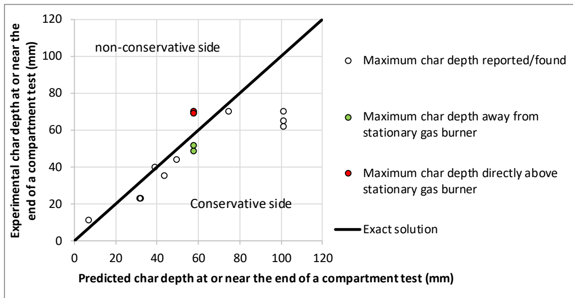
Figure 4: Maximum charring depths reported/found in compartment tests versus predicted charring rates (using the charring rate of eq.8)
