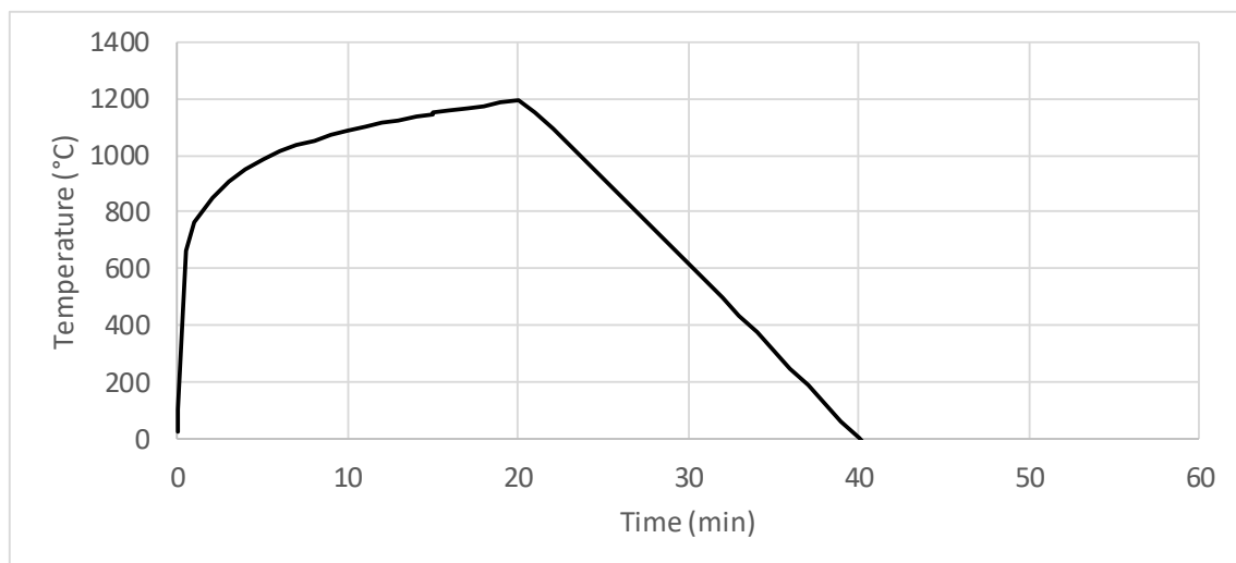
Figure A1: Predicted fire temperatures (corresponding to the charring rate according to eq.8)
