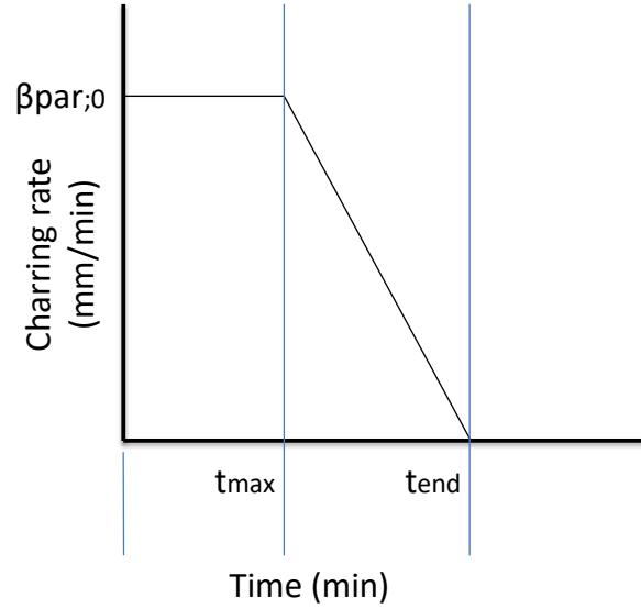
Figure 6: Proposed effective charring model
