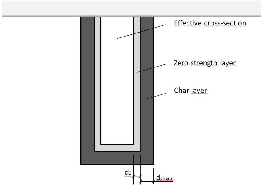
Figure 5: Effective cross-section of a beam in accordance with the reduced cross-section method
