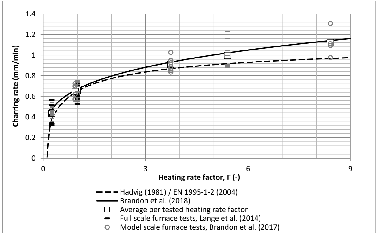
Figure 1: Charring rates during the fully developed stage of parametric fires
